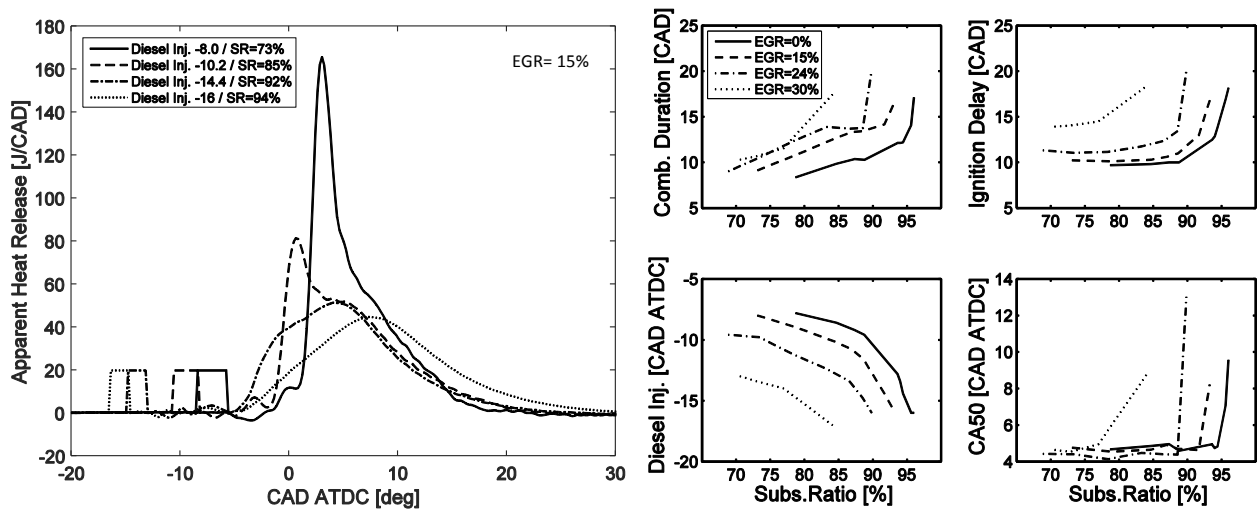
Figure 5: Heat release characteristics for different diesel injection timing [left] and EGR levels [right]
