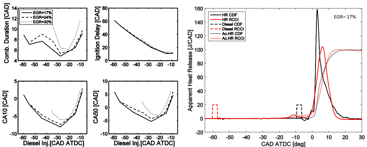
Figure 3: Heat release characteristics for SR=70% comparison between CDF and RCCI combustion
