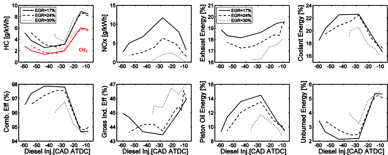
Figure 2: Emissions, efficiencies and energy balance for SR=70% transition from CDF towards RCCI combustion at different dilution levels
