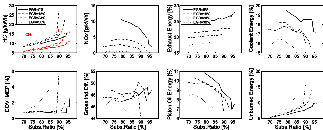
Figure 4: Emissions, efficiencies and energy balance for transition from CDF 70 to 95% SR at different dilution levels
