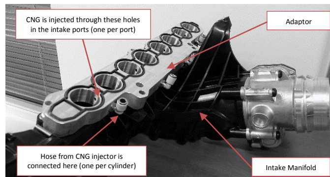
Figure 1: Adaptor plate for CNG injectors attached to intake manifold. Each injector supplies CNG to two different ports (one injector per cylinder)
