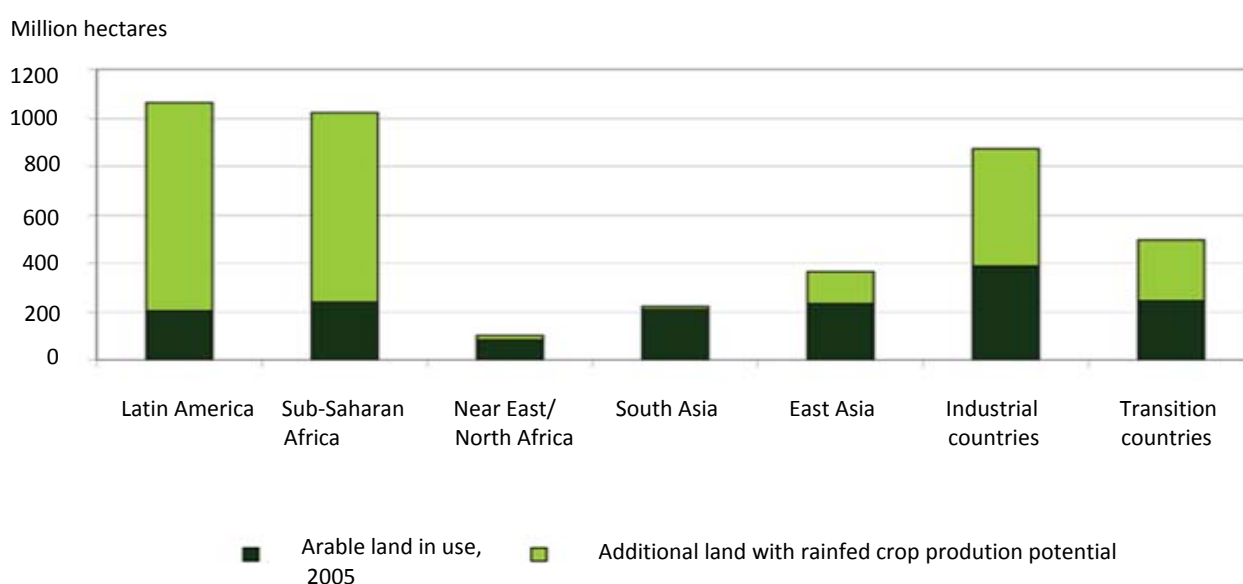
Figure 15. Distribution of land with rainfed crop potential by region Source: (Bruinsma, 2009). Adapted from (FAO, 2009a)
