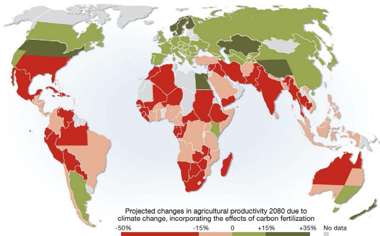
Figure 12. Projected losses in food production due to climate change by 2080
