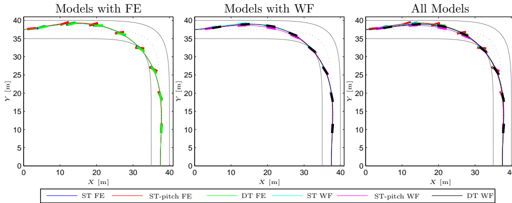
Figure 6. Time-optimal geometric trajectories in the 90°-turn obtained for the respective model configuration. The colored bars represent the vehicle heading every half second.
