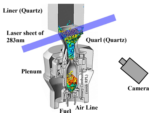
Figure 5.4: Schematic diagram of the experimental setup and of the full burner assembly.
