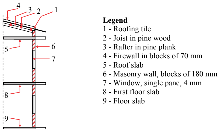
Figure 4.1. Building elements section.
