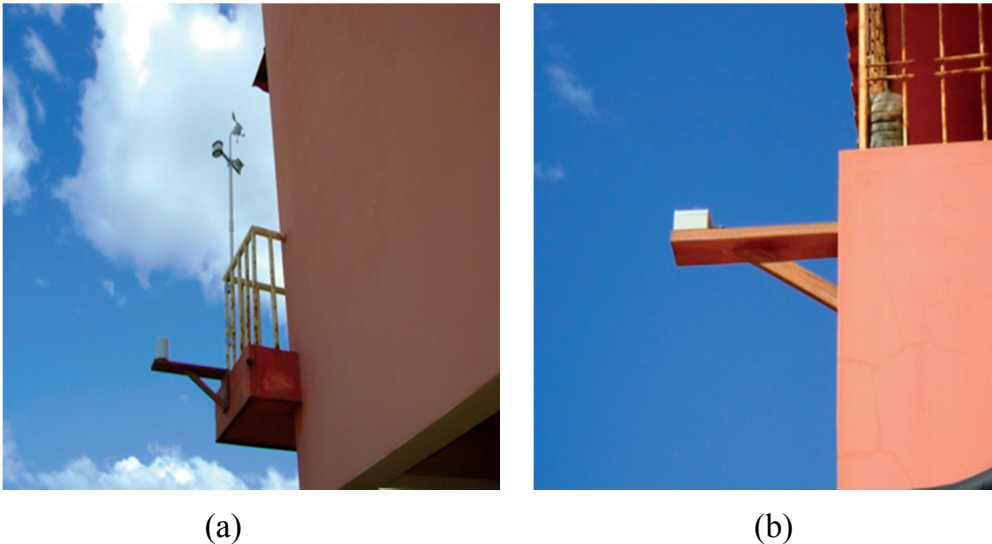
Figure 3.9: (a) Wind, temperature, humidity and rainfall sensors on the south side of the building. (b) Irradiance sensor on the north side of the building.
