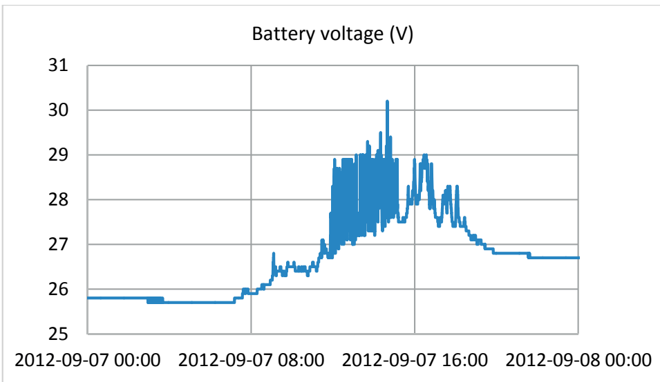
Figure 3.33: Battery voltage, 2012-09-07.
