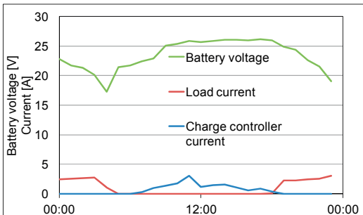
Figure 15. Battery voltage, load current and charge controller current on 2013-02-05.
