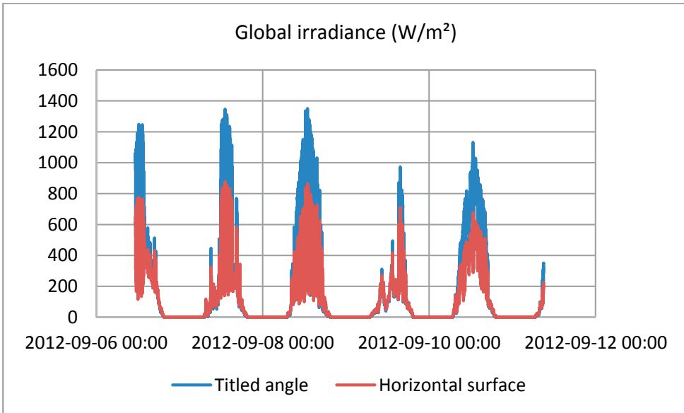
Figure 3.27: Global irradiance.
