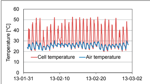
Figure 9. Air temperature and PV cell temperature during February 2013.
