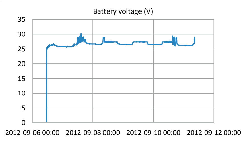
Figure 3.32: Battery voltage.
