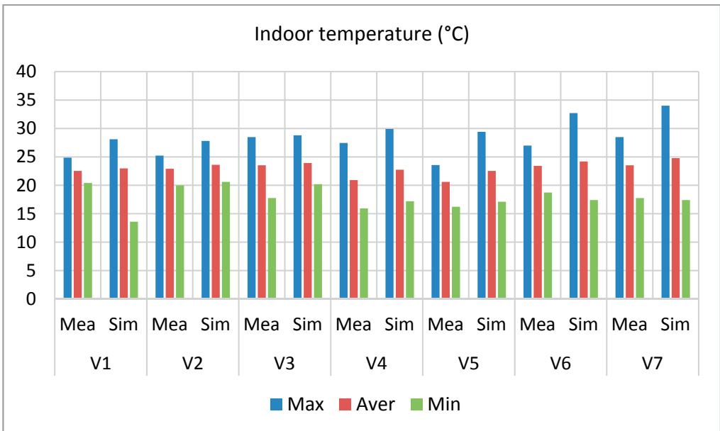
Figure 3.5(b): Indoor temperature per volume in July.
