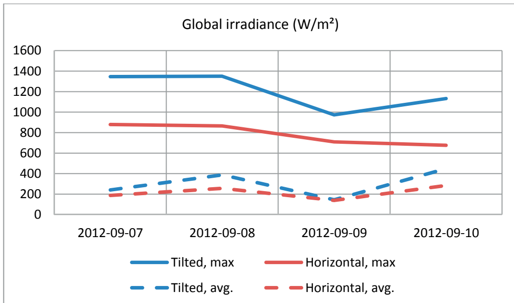
Figure 3.28: Global irradiance.
