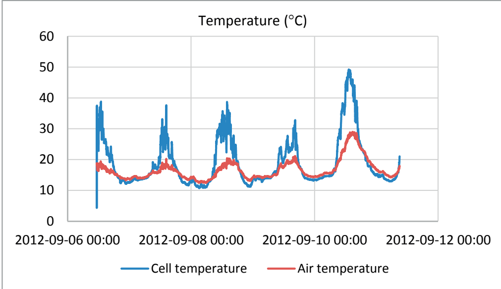
Figure 3.29: Cell and air temperatures.
