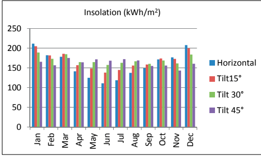
Figure 1. Monthly insolation in kWh/m 2 .
