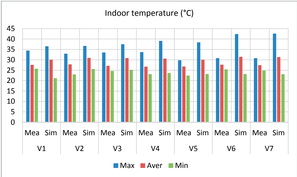
Figure 3.5(a): Indoor temperature per volume in January.
