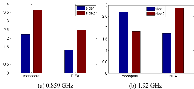
Fig. 7. Stand-alone SAR for antenna setups with different antenna types.
