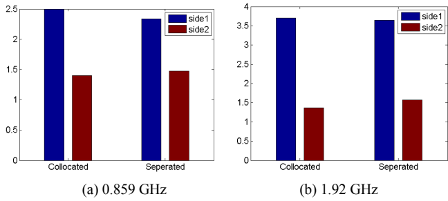
Fig. 3. Stand-alone SAR for co-located and separated antenna setups.
