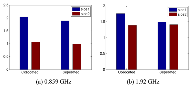
Fig. 5. Average simultaneous SAR for co-located and separated antenna setups.
