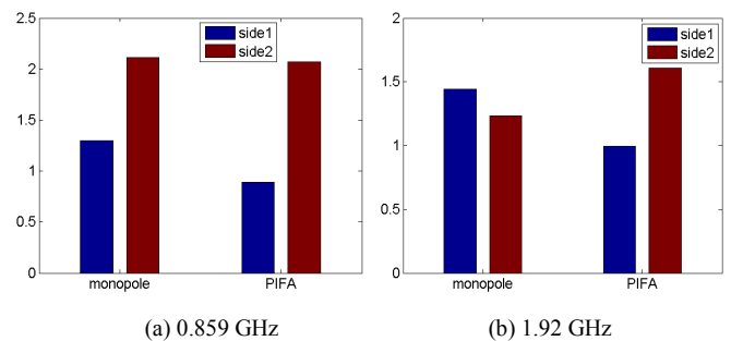
Fig. 9. Average simultaneous SAR for antenna setups with different antenna types.
