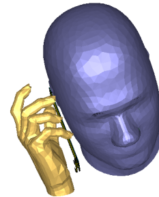
Fig. 6. Mobile handset with hand and head phantom.
