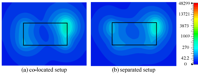
Fig. 4. Magnitude of E field distributions for different antenna setups in free space at 0.859 GHz.
