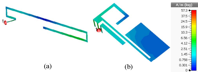
Fig. 8. Current distribution for monopole and PIFA antennas at 1.92 GHz.
