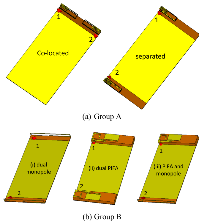
Fig. 1. Antenna configurations for (a) different antenna locations. (b) different antenna types.
