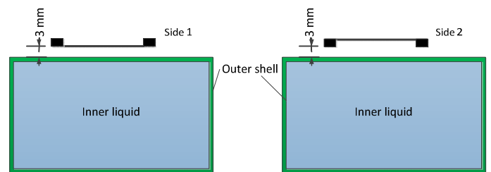
Fig. 2. The flat phantom and the position of the antennas.
