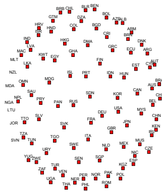
Figure 4.4: MDS-based visualization of gross trade flows between 100 countries, excluding the 8278 edges that represent bilateral gross trade
