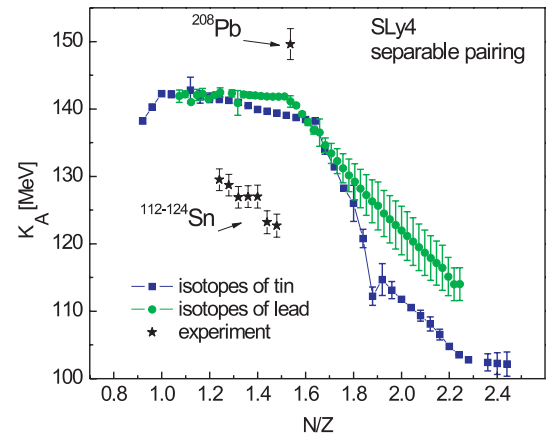
FIG. 9. (Color online) Incompressibility K_A calculated for the SLy4 functional and separable pairing force in tin (squares) and lead (circles) isotopes compared to the available experimental data. Theoretical results are plotted together with uncertainties pertaining to variations of the neutron strength parameter in the range of G_n = 631 \pm 150 \text{ MeV fm}^3 .
