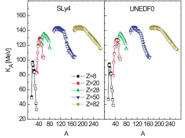
FIG. 4. (Color online) Incompressibility K_A calculated for the isotopic chains of semimagic nuclei with Z = 8, 20, 28, 50 , and 82 . Left and right panels show results obtained for the SLy4 and UNEDF0 functionals, respectively. Full (empty) symbols correspond to the zero-range (separable) pairing force.
