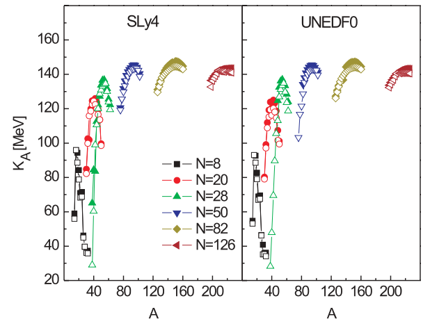
FIG. 5. (Color online) Same as in Fig. 4, but for the isotonic chains with N = 8, 20, 28, 50, 82 , and 126 .
