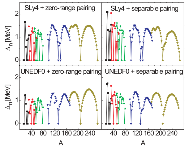
FIG. 1. (Color online) Neutron pairing gaps in the Z = 8, 20, 50 , and 82 isotopes (see the legend shown in Fig. 4). Upper and lower panels show results obtained for the SLy4 and UNEDF0 functionals, respectively. Left and right panels show results obtained for the zero-range and separable pairing, respectively.
