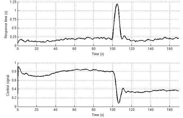
Figure 19. Performance of the LAC with step in observable traffic.
