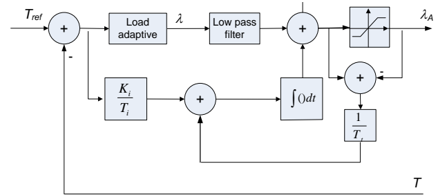
Figure 15. Load-adaptive controller (LAC)
