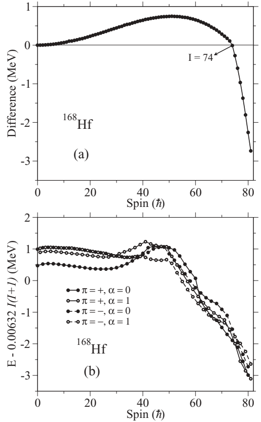
FIG. 10. (a) The difference between the reference energy based on the LSD model, with a moment of inertia calculated from a diffuse surface [25], and the standard I(I+1) reference for the ^{168}\text{Hf} nucleus. (b) The ^{168}\text{Hf} yrast energies relative to the standard I(I+1) reference. These energies, which are minimized in the (\varepsilon_2, \gamma, \varepsilon_4) space of deformation, cf. Fig. 7, are shown as a function of spin I for the four combinations of parity and signature, (+, 0) , (+, 1) , (-, 0) , and (-, 1) .
