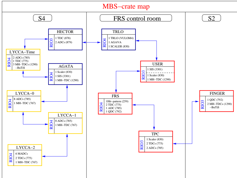
Figure 1: Schematic view of the location of the complex and widely distributed MBS DAQ system of the PreSPEC-AGATA campaign. Each of the eleven VME crates was linked with the trigger bus connection represented by the blue arrow. Each box represents a crate. Red contours denote the FRS sub-system, yellow the LYCCA sub-system and blue the AGATA sub-system. The BuTiS sign means that the MH-TDCs of the crates were synchronised with an external clock. Modules in each crate are listed according to their abbreviations (see text for details).
