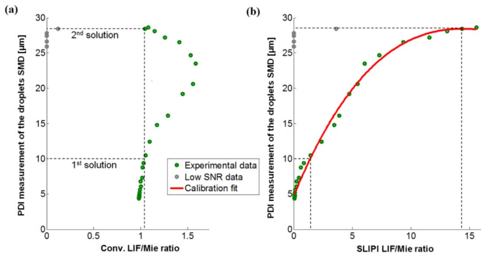
Fig. 28: Plots of the SMD values measured with PDA against the corresponding LIF/Mie ratio. In (a) the “conventional” case shows two SMD solutions for a single LIF/Mie ratio. In this case, the measurement cannot be calibrated. In (b) the SLIPI case shows a unique solution for each LIF/Mie ratio. This confirms the possibility of extracting a reliable calibration curve that can be used to deduce the absolute droplets SMD from Fig. 26(b).
