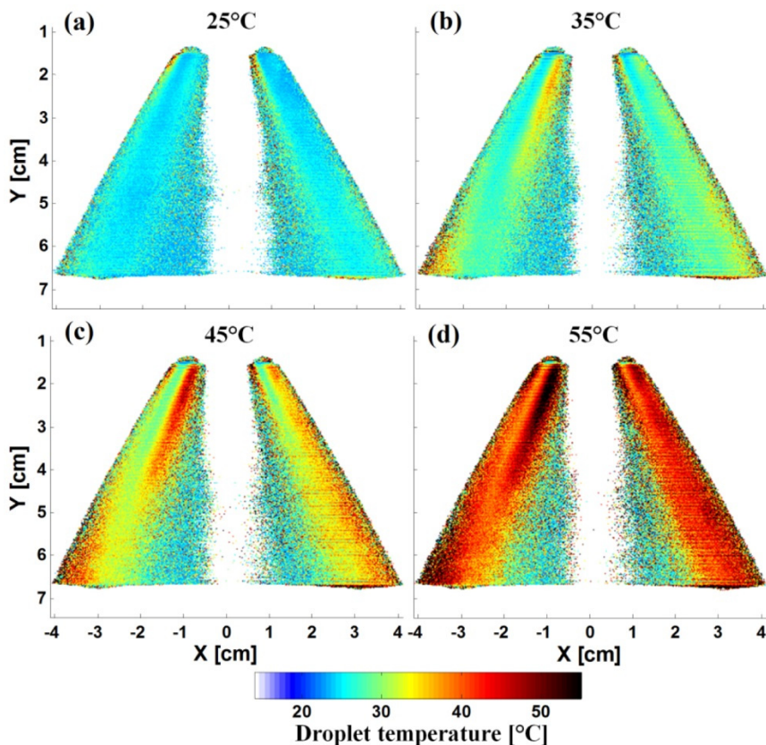
Fig. 38: Two-dimensional map of droplet temperature in a hollow-cone water spray at reference temperature varying between 25°C to 55°C. The spray cools down in its hollow region while the liquid located nearer to the nozzle orifice is hotter.
