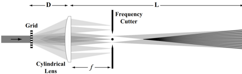
Fig. 23: Generation of the structured beam in fringe projection approach by letting the 1st order diffraction interference. Image from reference[16].
