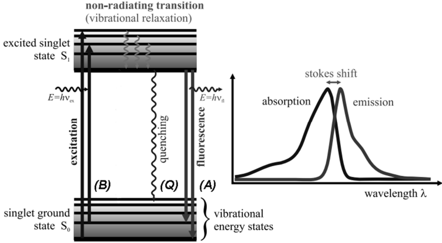
Fig. 12: Jablonski diagram and spectrum illustrating the processes involved in the creation of an excited state by optical absorption and subsequent emission of fluorescence. From reference [79].
