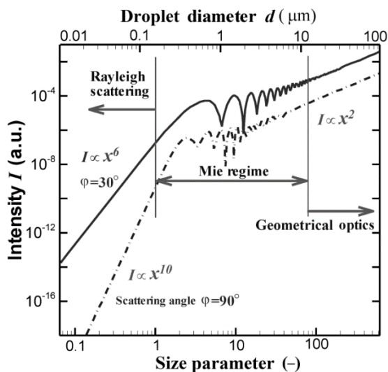
Fig. 9: Scattered intensity as a function of size parameter and droplet diameter. Based on the size parameter, three different regimes of light-droplet interaction can be identified. Adapted from reference [78].
