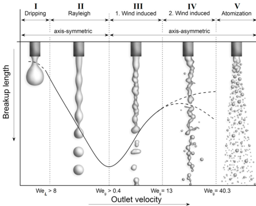
Fig. 2: Illustration of the breakup regimes of round liquid jets in the quiescent air. Impact of outlet velocity on breakup length of injected liquid from a circular nozzle; I: Dripping; II: Rayleigh breakup; III: First wind-induced breakup; IV: Second wind-induced breakup; V: Atomization. From reference [65].
