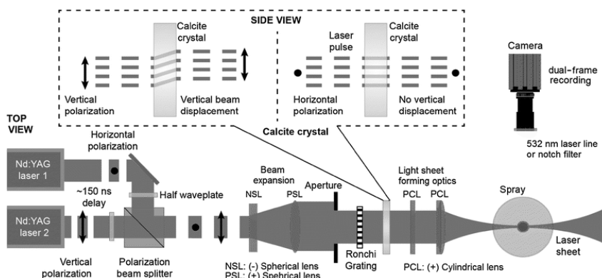
Fig. 39: The schematic of the 2p-SLIPI experimental setup for imaging transient sprays.
