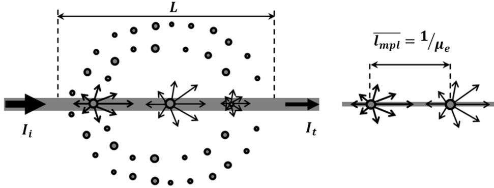
Fig. 13: Illustration of light extinction, and photon mean free path length.
