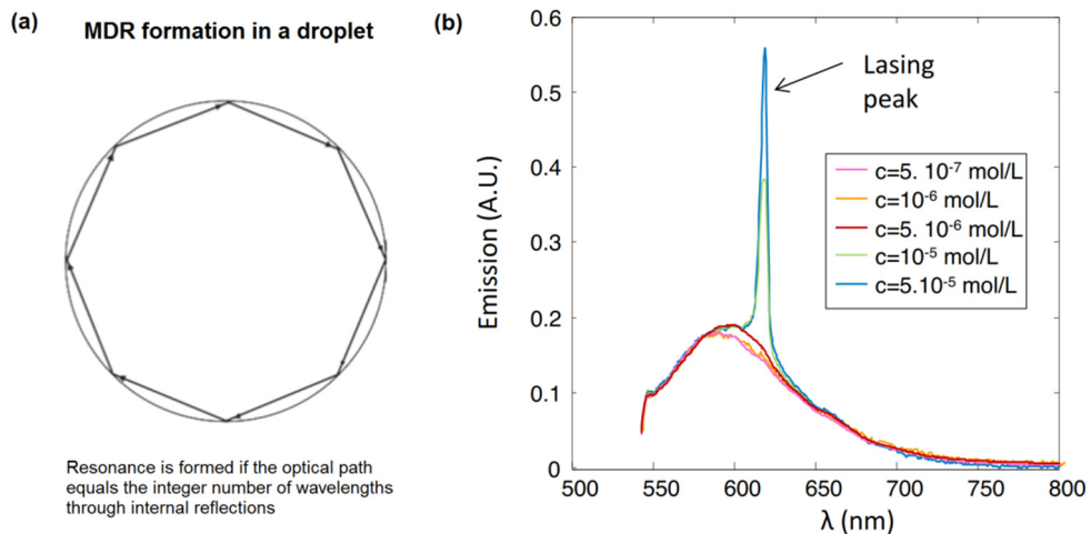
Fig. 21: (a) Illustration of MDR formation in a droplet. (b) The emission of a lasing peak inside the droplet at 620 nm wavelength. Plots are from reference [106].
