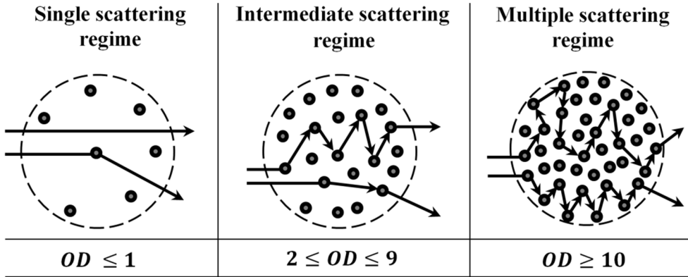
Fig. 14: Illustration of single and multiple scattering regimes estimated from the optical depth of the sample.
