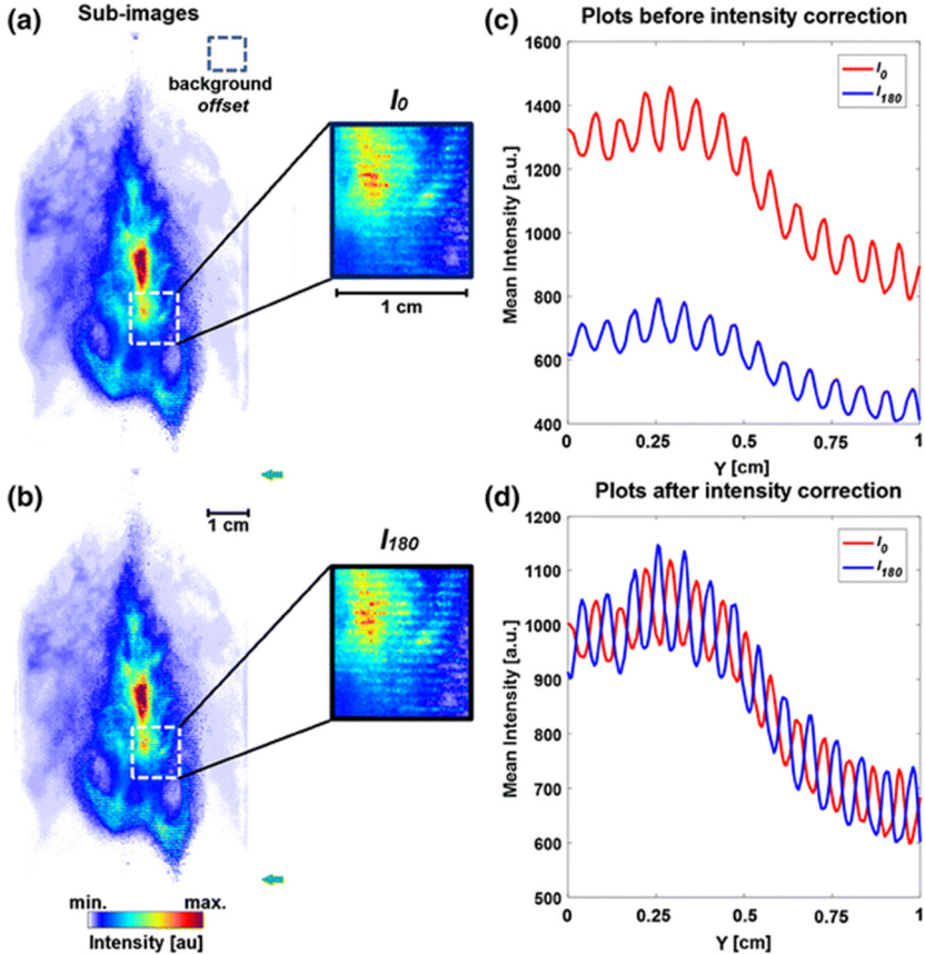
Fig. 40: Two modulated LIF sub-images of complementary phase are shown in (a) and (b). The plots of the mean intensity of I_0 and I_{180} from the indicated region (white-dashed box) are given in (c) without any intensity correction. The same plots are shown in (d) after the correction procedure for the variations in light intensity.
