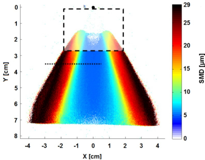
Fig. 29: Two-dimensional map of the absolute droplets SMD for a hollow-cone water spray running at 20 bar injection pressure. The result is obtained from SLIPI LIF/Mie after calibration with PDA data. The PDA measurements were performed at 3.5 cm below the nozzle tip, along with the black dot line the image.
