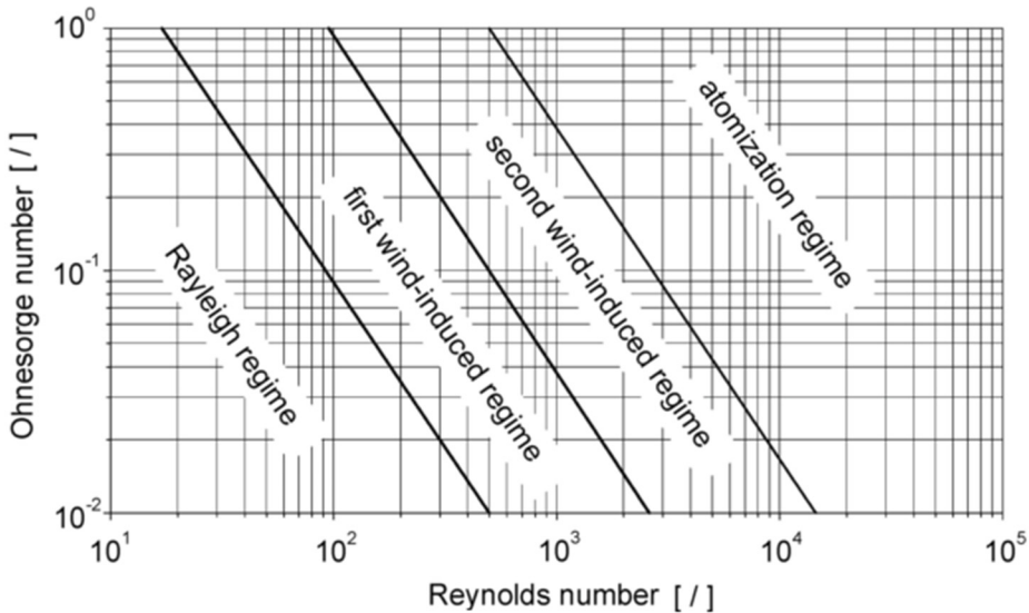
Fig. 3: The Ohnesorge diagram of a jet break-up. From reference [68].
