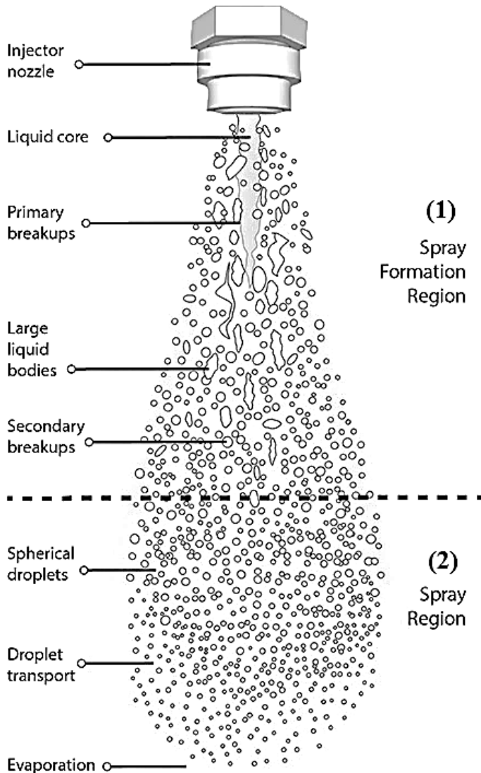
Fig. 4: Atomizing sprays can be categorized into two regions: the spray formation region (1), and the spray region (2). The first region consists of primary and secondary atomization. In the spray region (2), the spray is expected to be fully developed and most of the droplets are assumed to be spherical. Source: www.spray-imaging.com .
