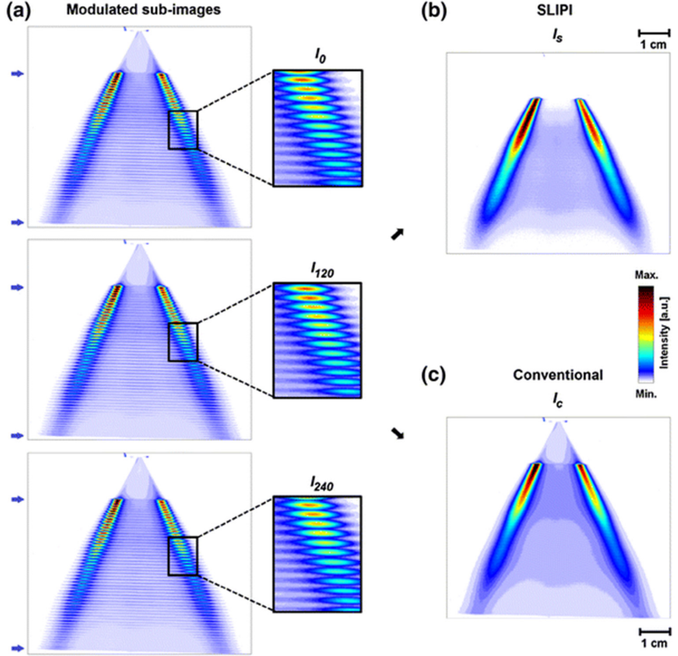
Fig. 1: Illustration of the 3p-SLIPI approach: The laser sheet having a sinusoidally-modulated intensity pattern along the vertical direction is intersecting a hollow-cone water spray. (a): Shows the three sub-images of the Mie scattered signal where the line-pattern is vertically moved one third of the spatial period. (b) and (c): Show the images of the SLIPI and “conventional” laser sheet, respectively, which are deduced using three sub-images in Eq. 2 and Eq. 3, respectively. The “conventional” image suffers from effects of multiple scattering, while in the SLIPI image those effects are reduced. From paper V.
