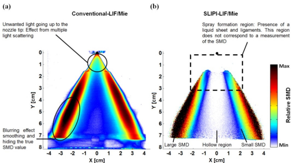
Fig. 26: Averaged images of the “conventional” LIF/Mie and SLIPI LIF/Mie, in (a) and (b) respectively, representing the relative SMD of droplets distribution. Effects from the multiple light scattering can be seen on the “conventional” SMD image.
