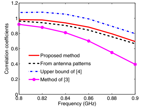
Fig. 9. Magnitude of correlation coefficient for the monopole array on mobile chassis.
