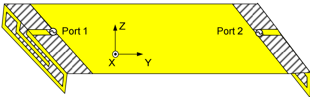
Fig. 7. Geometries of the folded monopole antennas on mobile chassis. Detailed dimensions are available in [9].
