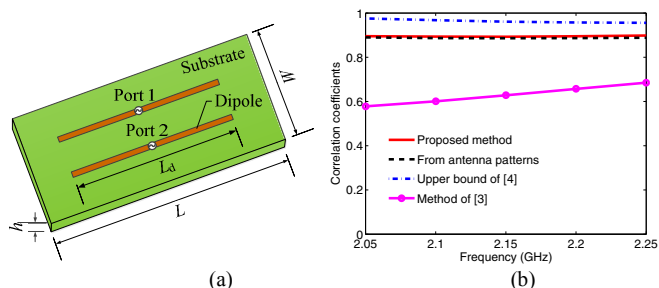
Fig. 3. (a) Geometries of the dual-dipole array. The dimensions are: W = 40 mm, L = 100 mm, h = 2 mm, L_d = 44 mm. (b) Magnitude of correlation coefficient for the dual-dipole array over the operating band.
