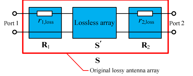
Fig. 2. Cascade network model for a lossy dual-dipole array.
