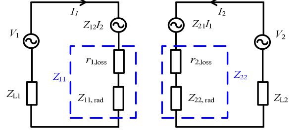
Fig. 1. Equivalent circuit model of a lossy dual-dipole array.
