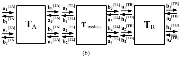
Fig. 6. (a) Cascade network model for a lossy four-element array; (b) Relationship between the incoming and outgoing waves.
