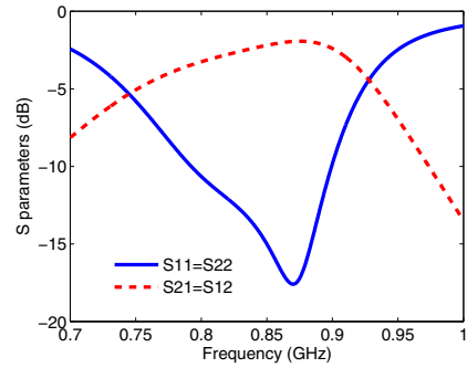
Fig. 8. The S parameters of the two folded monopole antennas on the mobile chassis.
