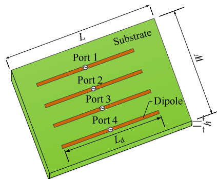
Fig. 4. Geometries of the four-dipole array. The dimensions are: W = 80 mm, L = 100 mm, h = 2 mm, L_d = 44 mm.
