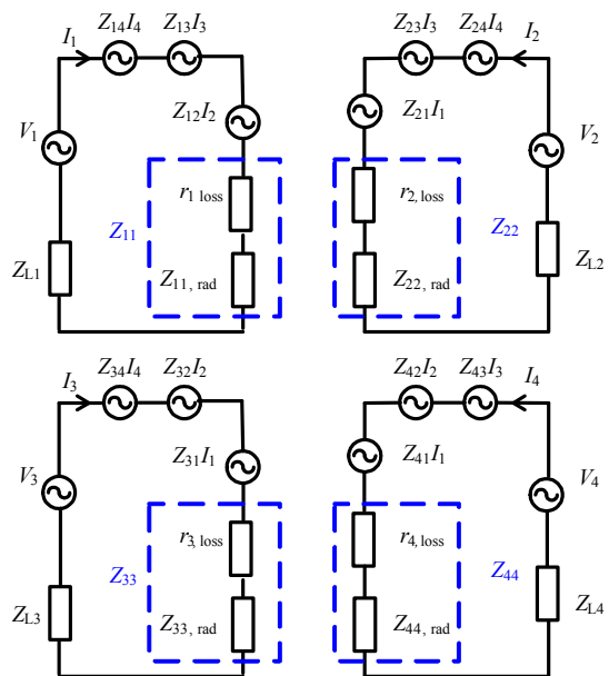
Fig. 5. Equivalent circuit model of a lossy four-dipole array.
