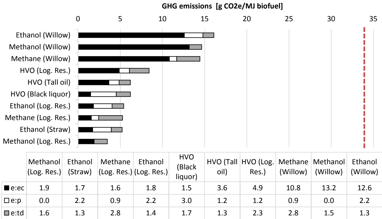
Figure 3. GHG emissions of extraction and cultivation efforts (e:ec), production and conversion of feedstock (e:p) and transportation and distribution (e:td) according to the EU RED methodology for the biofuels methanol, methane, ethanol and HVO with different feedstock and conversion pathways. The dashed line indicates GHG emissions of 34 g CO 2 e/MJ biofuel, corresponding to a 60% GHG emission saving compared to fossil fuel reference used in the EU RED.
