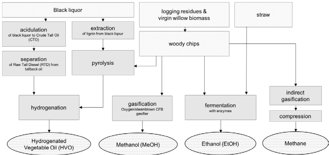
Figure 1. Schematic overview over biomass, pathways and biofuels considered in this report.
