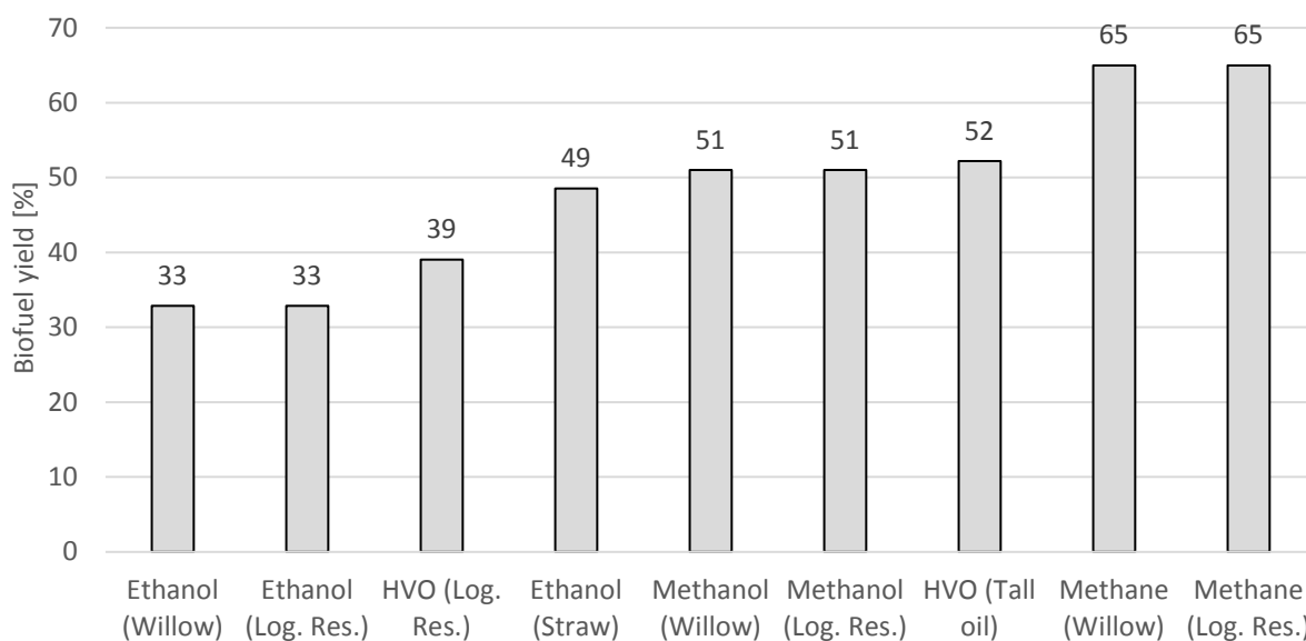
Figure 4. Biofuel yield (MJ biofuel per MJ biomass feedstock (LHV)).
