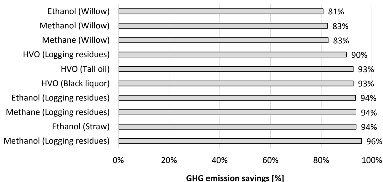
Figure 2. Aggregated results on GHG emission savings for the biomass-biofuels pathways investigated.
