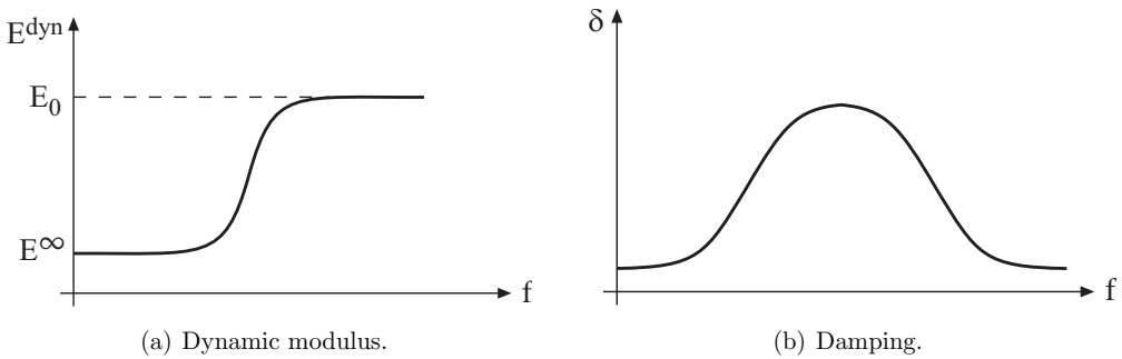
Figure 3.16: Dynamic measurements of linear viscoelastic materials.
