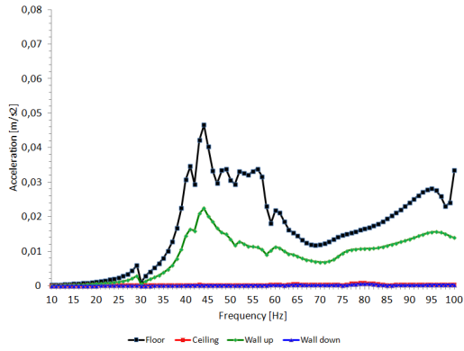
Fig. 8 - Case A widthwise. Acceleration magnitudes evaluated on the floor, ceiling, upper and bottom walls (left) and acceleration magnitudes evaluated on top and bottom of the Syldyn (right).
