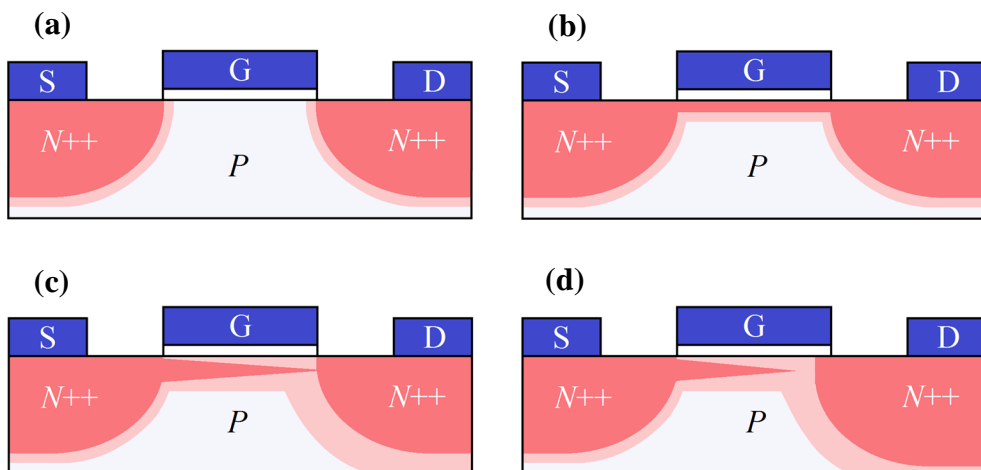
Fig 1.6. Schematic illustrations of different biasing conditions of a planar MOSFET. The device has metal deposited in direct contact with highly doped ( N_{++} ) regions at the source, S , and the drain, D . The lower doped channel ( P ) is controlled by the potential in gate, G , where the metal contact is separated by a dielectric film. (a) No gate bias is applied and there is no conducting path between S and D . (b) A gate bias beyond threshold is applied, meaning that an inversion layer is formed at the channel surface. (c) The gate is biased at a higher potential than in (b) and the potentials of S and D differ to an extent corresponding to channel pinch-off. (d) The potential difference between S and D is increased beyond pinch-off and thus the effective channel length is reduced.
