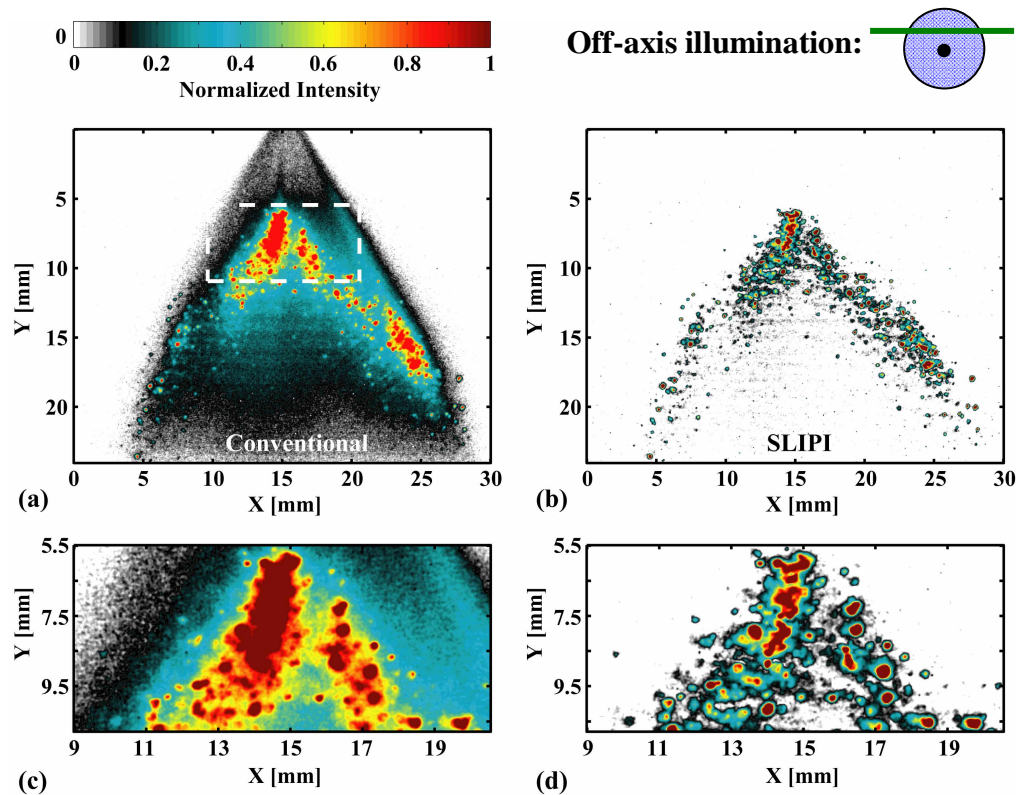
Fig. 5. Comparison between the conventional planar Mie imaging and SLIPI. The planar illumination is \sim 5 mm off-axis (behind) from the nozzle centre. Each image corresponds to an average of 50 triple images. A magnified area indicated by the dashed lines in (a) is illustrated for the conventional and the SLIPI image in (c) and (d) respectively.
