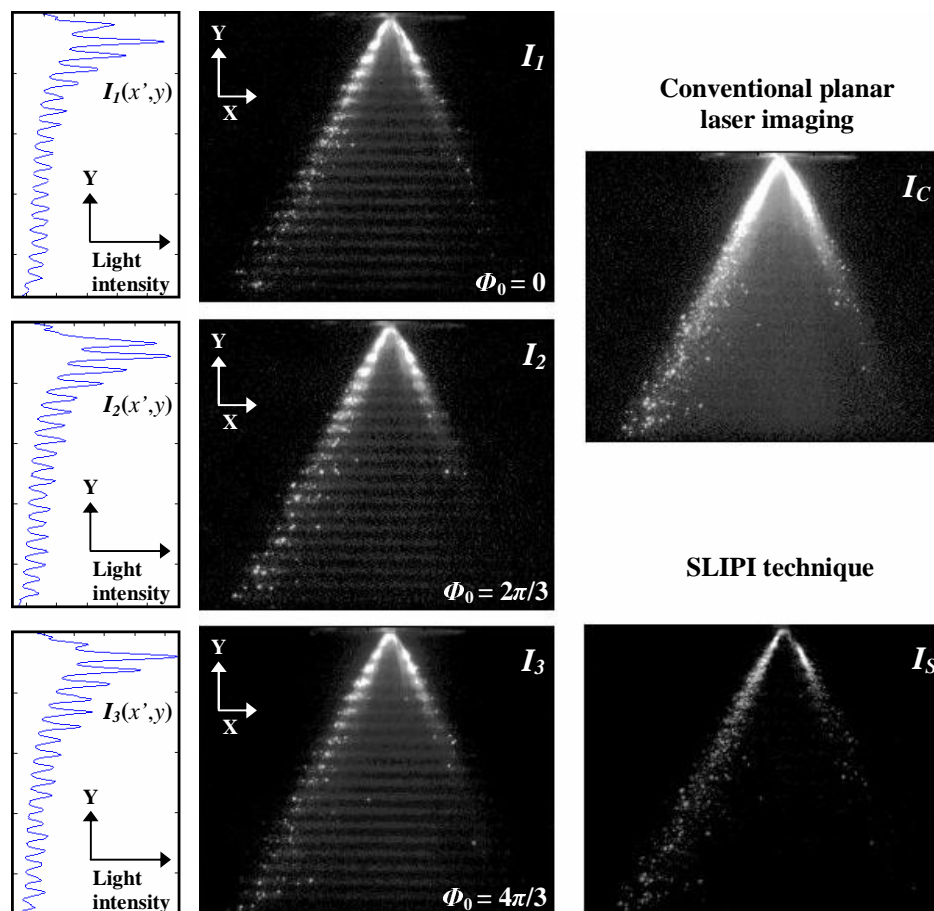
Fig. 2. Illustration of the SLIPI technique: 3 successive images are taken by illuminating different parts of the spray after shifting the spatial modulation one third of a period. When summing up the images, the conventional I_C is obtained, whereas, when extracting the absolute value of the differences between the images, a new image I_S is formed without most of the multiple light scattering. The modulated signal I(x',y) is given for each image on the left side of the figure, at a given distance x = x' .
