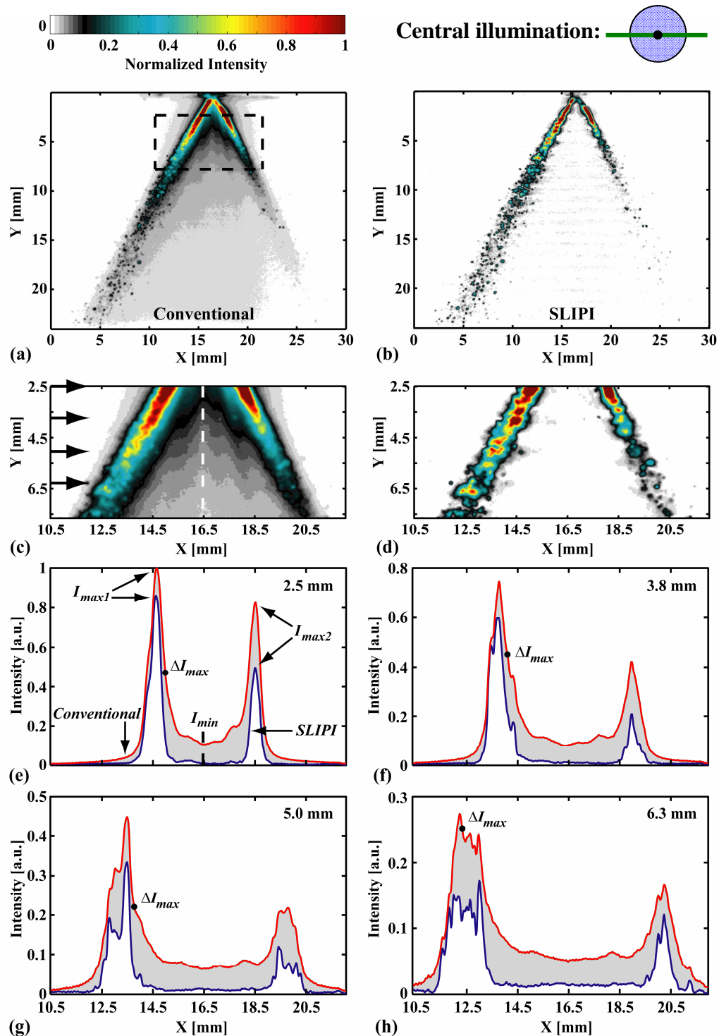
Fig. 4. Comparison between the conventional planar Mie imaging and SLIPI for the central illumination. Each image corresponds to an average of 50 triple images. A magnified area indicated by the dashed lines in (a) is illustrated for the conventional and the SLIPI image in (c) and (d) respectively. The intensity profile along the horizontal direction is given at four vertical positions indicated by the arrows in (c).
