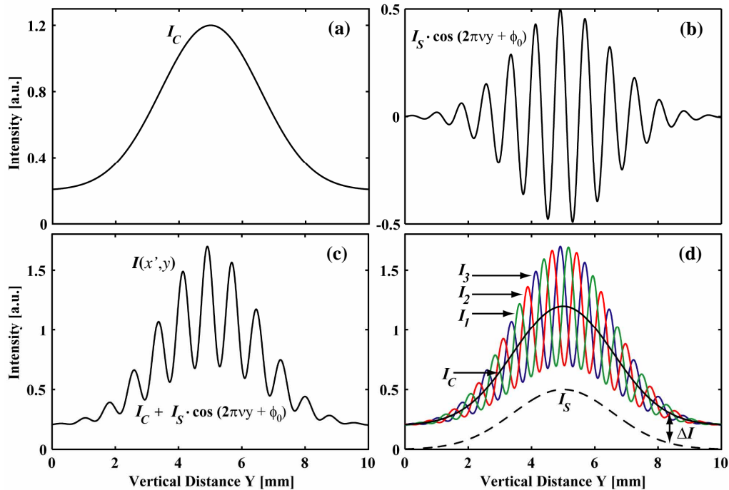
Fig. 1. Illustration of the conventional (a) and modulated components (b) with the resultant signal I(x',y) in (c) for a given distance x = x' . Using three signals I(x',y) each shifted one third of a period relative to each other, the SLIPI signal I_S can be extracted as seen in (d).
