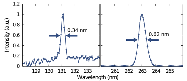
FIG. 7. Full-width half maximum linewidth of a peak measured at 131 nm and 263 nm is used to estimate the pulse length. Both spectra are normalized. The noise is less prominent on the fundamental due to higher intensity.
