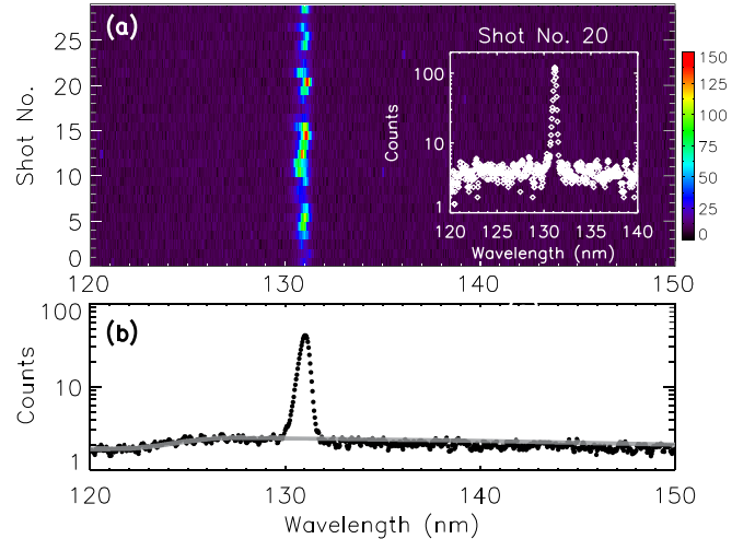
FIG. 3. A series of single shots taken at the 2nd harmonic at 131 nm (a) and the time averaged intensity over these 30 shots (b). A single shot spectrum is depicted in the inset. The calculated incoherent undulator harmonic was fitted for the pulse energy calibration (gray line in (b)). These measurements were done before stability improvements on laser-electron overlap.
