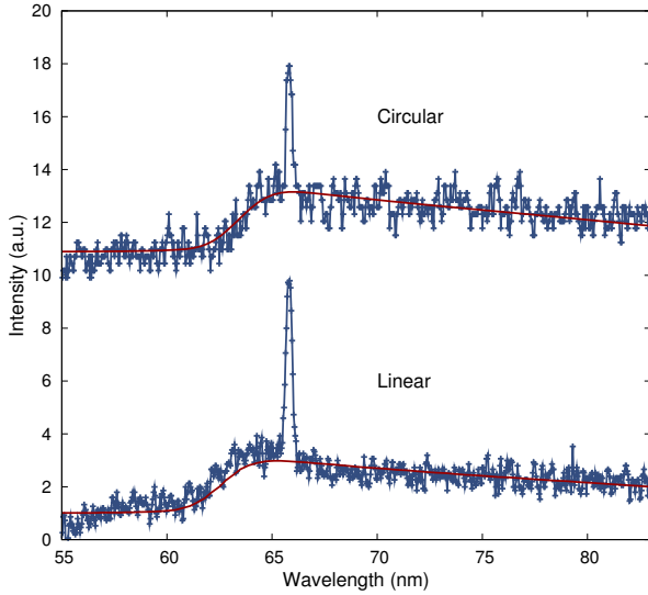
FIG. 5. Coherent 4 th harmonic in circular and linear polarization. The full lines indicate the expected incoherent undulator harmonic according to SPECTRA simulations. The coherent gain is of the same order of magnitude in both cases and its difference is within the margins of overall stability fluctuations of the system.
