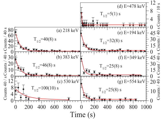
FIG. 7. (Color online) \beta -delayed \gamma -ray gated time spectra for the transitions 218, 383, 530, 478, 194, 349, and 554 keV associated with decay in ^{194}\text{Os} for different correlation times \Delta t(\text{implant} - \beta) = 0 \rightarrow 1000 s from the current work. By using a least squared fit the data were fitted to a single exponential decay function plus a constant background level.
