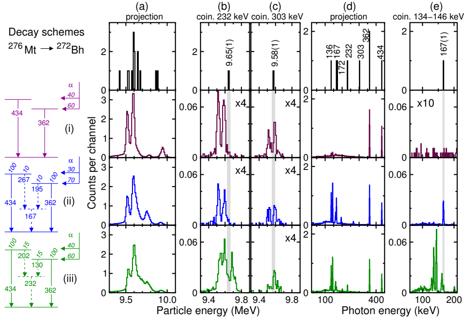
Fig. 4. Color on-line: Experimental (top row) and normalized simulated [27] particle and photon spectra based on presumed decay schemes of the 4 th -generation ^{288}_{115}\text{Mt} decay step ^{276}\text{Mt} \rightarrow ^{272}\text{Bh} . From left to right, the columns provide the decay schemes, the total particle spectra, coincidence spectra with [230,234]-keV and [301,305]-keV photons, the total photon spectrum, and a photon spectrum in coincidence with ^{272}\text{Bh} K_\alpha X rays, i.e. with [134,146]-keV photons.
