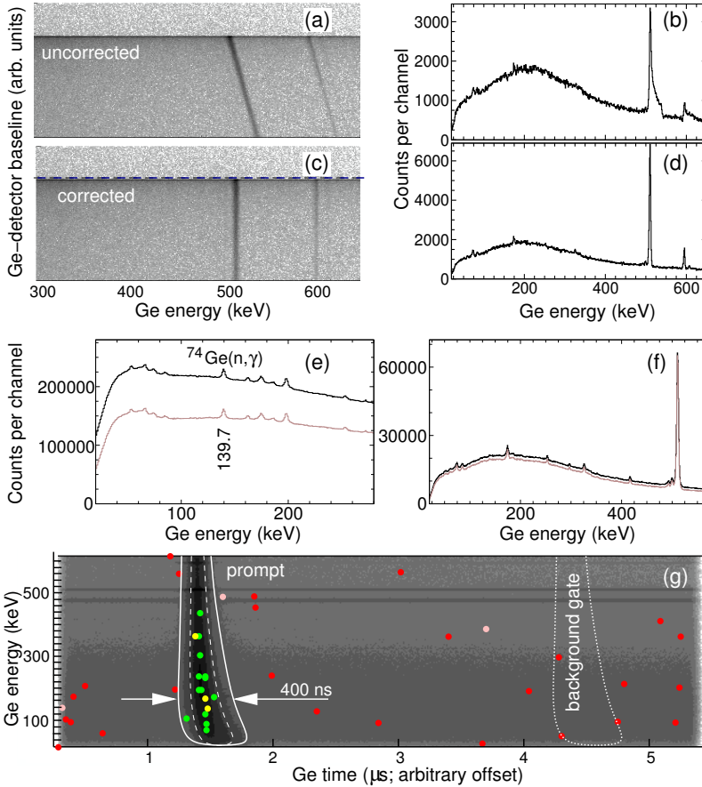
Fig. 1. Color on-line: Panels (a) and (c) provide uncorrected and corrected two-dimensional plots of baseline vs. energy for the central Ge detector of the cluster detector positioned behind the TASI Spec implantation DSSSD [23, 27]. Spectra in panels (b) and (d) are the corresponding projections. Data stems from both beam-on and beam-off periods. Panels (e) and (f) show sum spectra during beam-on and beam-off periods without a prompt coincidence condition, and only during beam-off and with a prompt coincidence requirement, respectively. The gray spectra require the Ge-detector baseline being below the dashed line in panel (c). Panel (g) provides the correlation between Ge-detector energies and Ge-detector times measured with respect to the event trigger, i.e. an energy-corrected timing signal from the implantation DSSSD, during beam-off periods. See the text for more details.
