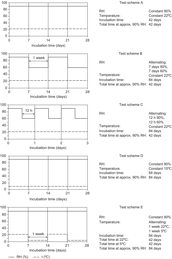
Fig. 1. Test schemes.
