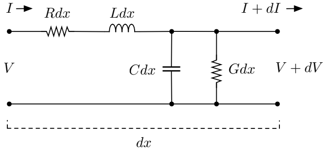
Figure 1.4: A uniform transmission line segment of length dx . The voltage and current at the input of the line segment are represented by V, I , respectively. The line segment can be thought of as a dissipative low-pass filter.
