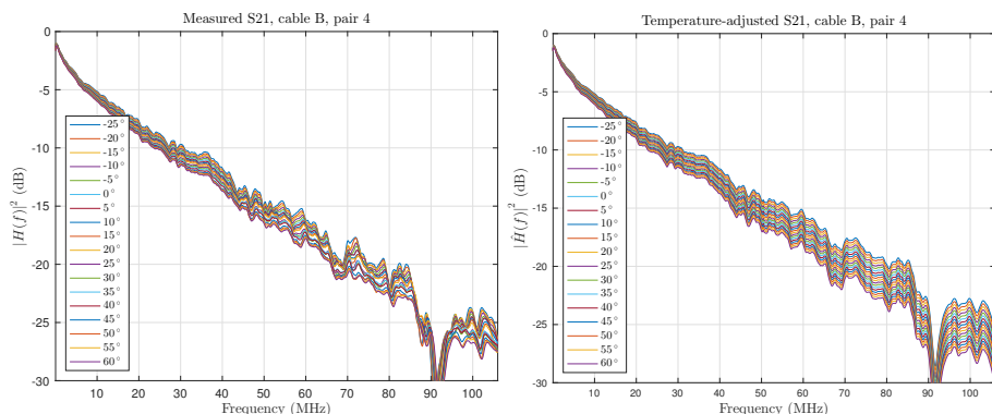
Figure 7.8: A comparison of the magnitudes of transfer functions for measured data (left side) and the estimate obtained using (7.11) (right side), for pair 4 in cable B.
