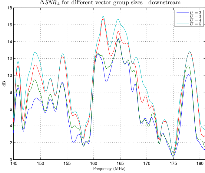
Figure 2.6: \Delta\text{SNR}_4 for different vectoring group sizes in downstream direction. Residual crosstalk increases with the number of lines.
