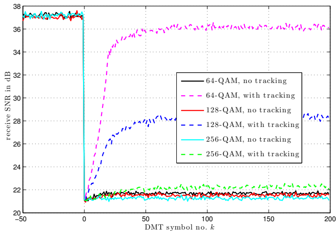
Figure 2.7: Receive SNR of user u = 4 with and without tracking for 64-QAM, 128-QAM, and 256-QAM. For k \geq 1 , a termination change from 100 Ohm to open on the alien line causes a sudden change in the channel matrix. The SNR results shown are averaged over 1000 simulation runs.
