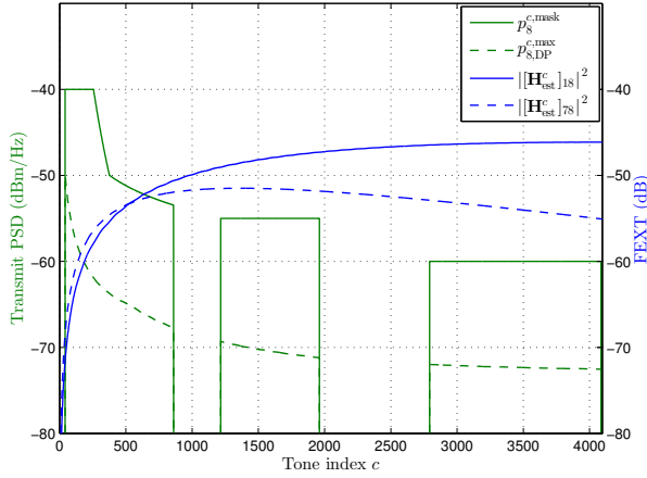
Figure 6.8: Left axis: transmit PSD mask and transmit PSD of user no. 8. Right axis: squared FEXT coupling magnitude from user no. 8 to users no. 1 and no. 7 ( q = 2\text{ dB} , \xi = 5\% ).
