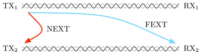
Figure 1.5: A schematic description of NEXT and FEXT between two pairs. For near-end crosstalk the source of interference and victim are connected at the same cable end. For far-end crosstalk the opposite is true.
