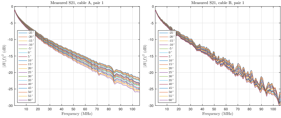
Figure 7.2: Attenuation for pair 1 on both cables. In cable A the spread between lowest and highest temperatures is higher, while overall attenuation at high frequencies is lower. Cable B presents a smaller spread but significant ripples on higher frequencies, suggesting a lower quality of construction.
