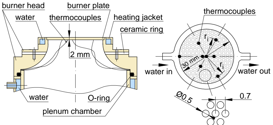
Figure 2.5: Cross-section and top view of the heat flux burner head designed by Eindhoven University of Technology.
