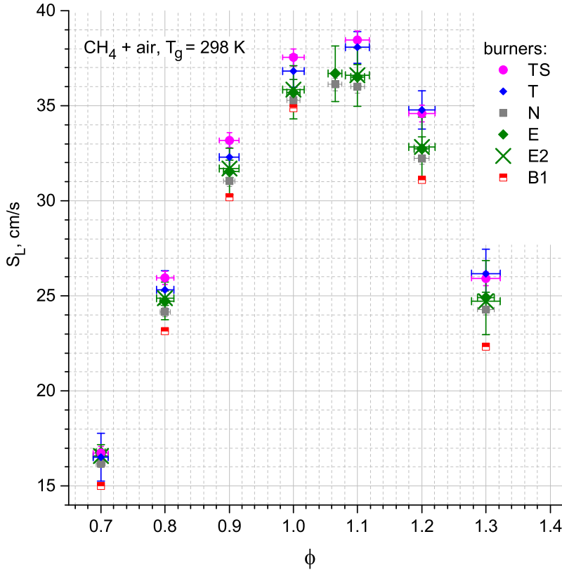
Figure 2.17: \text{CH}_4 + air burning velocity measured with different burners in Lund. The values are corrected for the surface area A .
