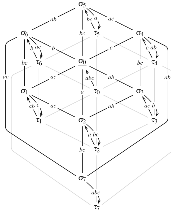
Fig. 5 The EPM denoted \mathbf{E}_0 , representing the joint perception of the occurrence of an accident for three agents a, b and c . All \sigma_k actions have \text{post}(\sigma_k) = A ; for all \tau_k , \text{post}(\tau_k) = \top . Grey links are only for presentation; they mirror the labels above. Links implied by transitivity are omitted, e.g. between \sigma_6 and \sigma_4 for a . In essence, \mathbf{E}_0 captures (1) that the accident in fact occurs, (2) that this is ambiguous for every agent, who all find it more plausible that it does occur and (3) that no agents learns anything about others' perception of the event, except that all have an opinion as to whether or not the accident occurred
