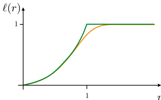
Figure 5.1: A robust loss function (orange) as suggested in [7], and the truncated L_2 -error (green) which can be optimized using the proposed framework; in this case truncated at \epsilon = 1 .
