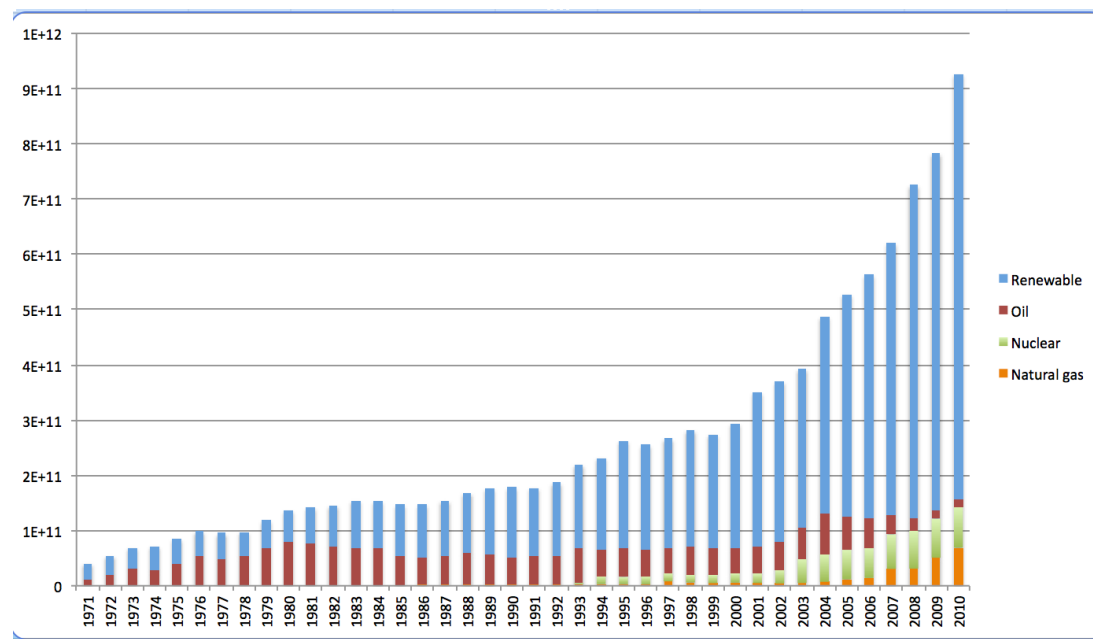
Figure 5. Electricity production from non-coal sources in China 1971-2010, kWh/year
