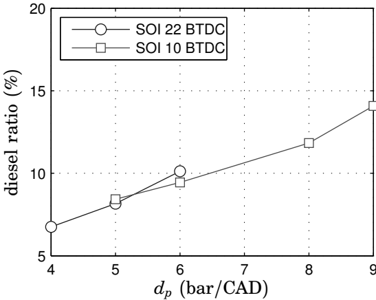
Figure 5.8 Diesel ratio required to keep a certain d_p for the two operation modes tested at 9.2 bar BMEP. With pure diesel operation, average d_p was 4.0 bar/CAD.
