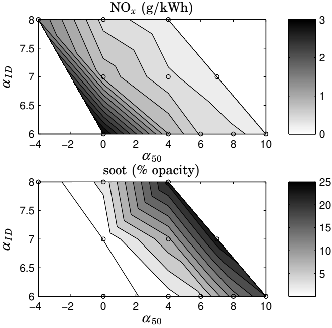
Figure 6.3 Emissions of NO x and soot mapped according to α 50 and α ID in steady-state operation. Circles represent measurement points, intermediate values are obtained by linear interpolation.
