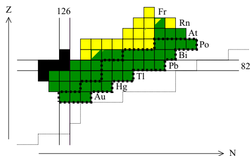
FIG. 1. (Color online) Nuclear region investigated in the present experiment. Residues formed in the fragmentation reaction are delimited by a thick dot-dashed line, whereas decay successors lie outside. Green (gray) and yellow (light gray) boxes stand for \beta and \alpha emitters, respectively. Stable nuclei are marked by black squares. The black dashed line shows the limit of nuclei so far synthesized.
