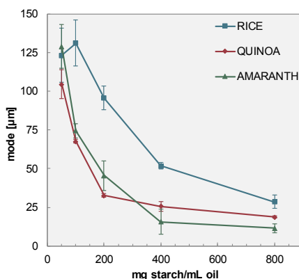
Fig. 20. The effect of starch type, concentration and level of OSA modification on emulsions' droplet size (mode of D_{4,3} ). Data reported from Marefati, Wiege et al. 2017 [39].
