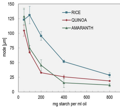
Fig. 5. Particle size (mode of D[4,3]) for 3.0% OSA modified starch emulsions.
