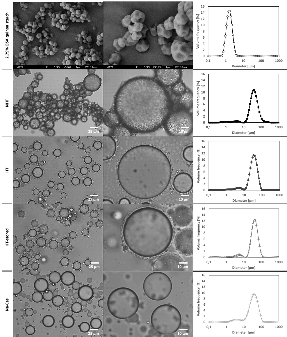
Fig. 29. SEM micrographs of quinoa starch granules and particle size distribution ( D_{4,3} ) of starch granules (top row), light microscopy micrographs and particle size distribution of non-heat treated emulsions (2nd row), light microscopy micrographs and particle size distribution of heat treated emulsions (3rd row), light microscopy micrographs and particle size distribution of heat treated and stored emulsions, (4th row) and light microscopy micrographs and particle size distribution of protein stabilized emulsions (bottom row), n=6 .
