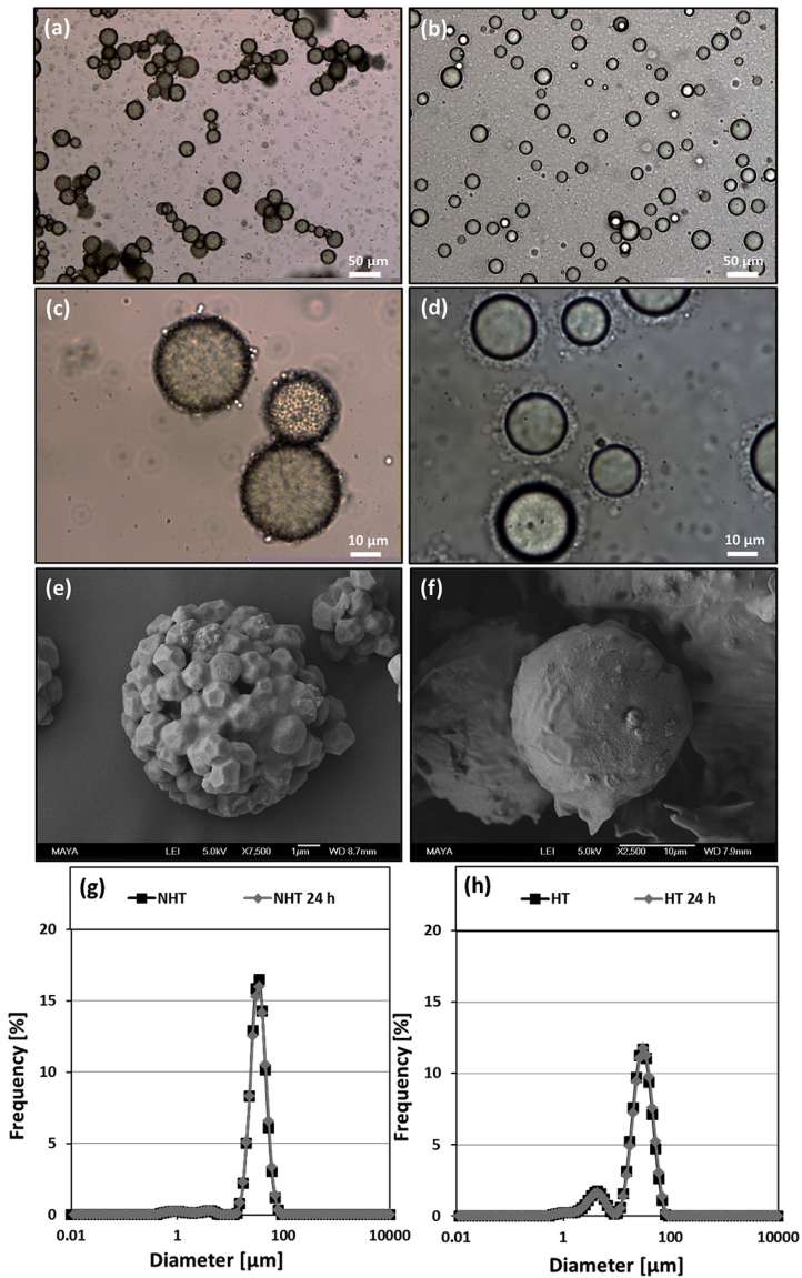
Fig. 5. (a) Light microscopy image of non-heat treated emulsion (NHT), (b) Light microscopy image of heat treated emulsion (HT), (c) Light microscopy image of non-heat treated emulsion (NHT) dried starch granule stabilized emulsion, (d) Light microscopy image of heat treated emulsion (HT) dried starch granule stabilized emulsion, (e) Scanning electron microscopy image of non-heat treated (NHT) dried starch granule stabilized emulsion, (f) Scanning electron microscopy image of heat treated (HT) dried starch granule stabilized emulsion, (g) Particle size distribution ( D_{4,31} ) for non-heat treated emulsion for fresh emulsions (NHT) and after 24 h (NHT 24h ), n = 6 , (h) Particle size distribution for non-heat treated emulsion for fresh emulsions (HT) and after 24 h (HT 24h ), n = 6 .
