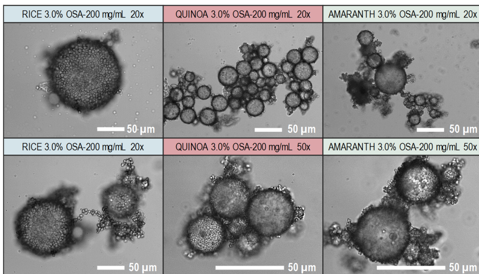
Fig. 19. Micrographs of emulsions stabilized by different types of starches with OSA modification level of 3%, reported from Marefati, Wiege et al. 2017 [39].
