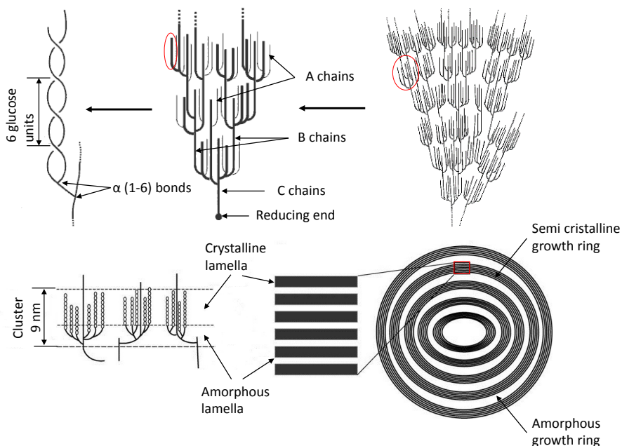
Fig. 9. Different structural levels of starch granules, adapted from Tester, Karkalaset al. 2004 [78] and Parker and Ring, 2001 [81]. The alternating crystalline and amorphous layers containing amylopectin double helices and branch respectively.
