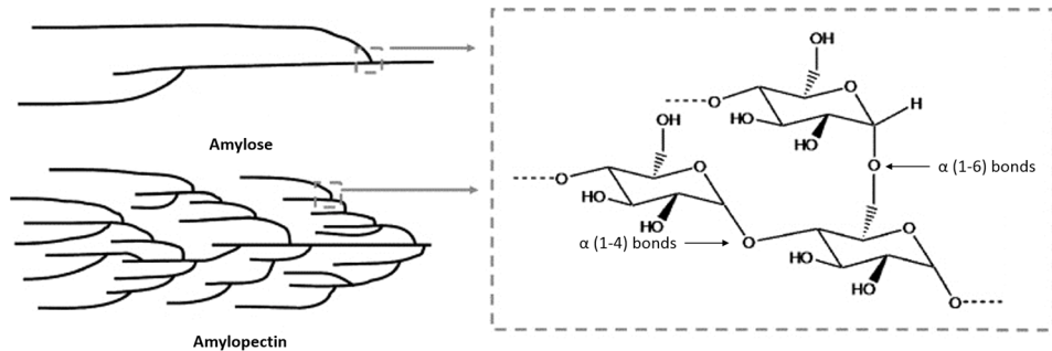
Fig. 8. Chemical structure of amylose and amylopectin. Fig. from Sweedman, Tizzotti et al. 2013 [75].
