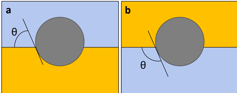
Fig. 6. Schematic representation of contact angle for (a) when lower than 90^\circ , oil-in-water emulsions are formed and (b) when higher than 90^\circ , water-in-oil emulsions are formed.
