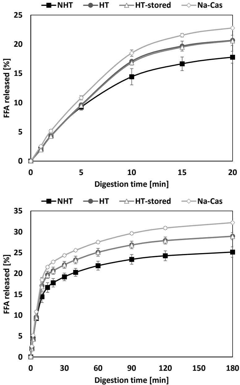
Fig. 4. The amount of FFA% produced for the different emulsions during the initial 20 min in vitro intestinal lipolysis (top), the amount of FFA% produced for the different emulsions during the 3 h in vitro intestinal lipolysis (bottom). Error bars represents standard deviation of the mean, n=3.
