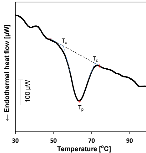
Fig. 10. DSC thermogram for gelatinization temperature of quinoa starch in phosphate buffer (5 mM, 0.2 M NaCl, PH 7). Fig. from Marefati, Bertrand et al. 2017 [51].
