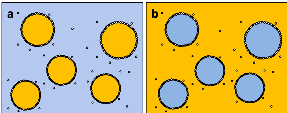
Fig. 5. Schematic representation of Pickering emulsions (a) oil-in-water (O/W) and (b) water-in-oil (W/O) Pickering emulsions stabilized by solid particles.
