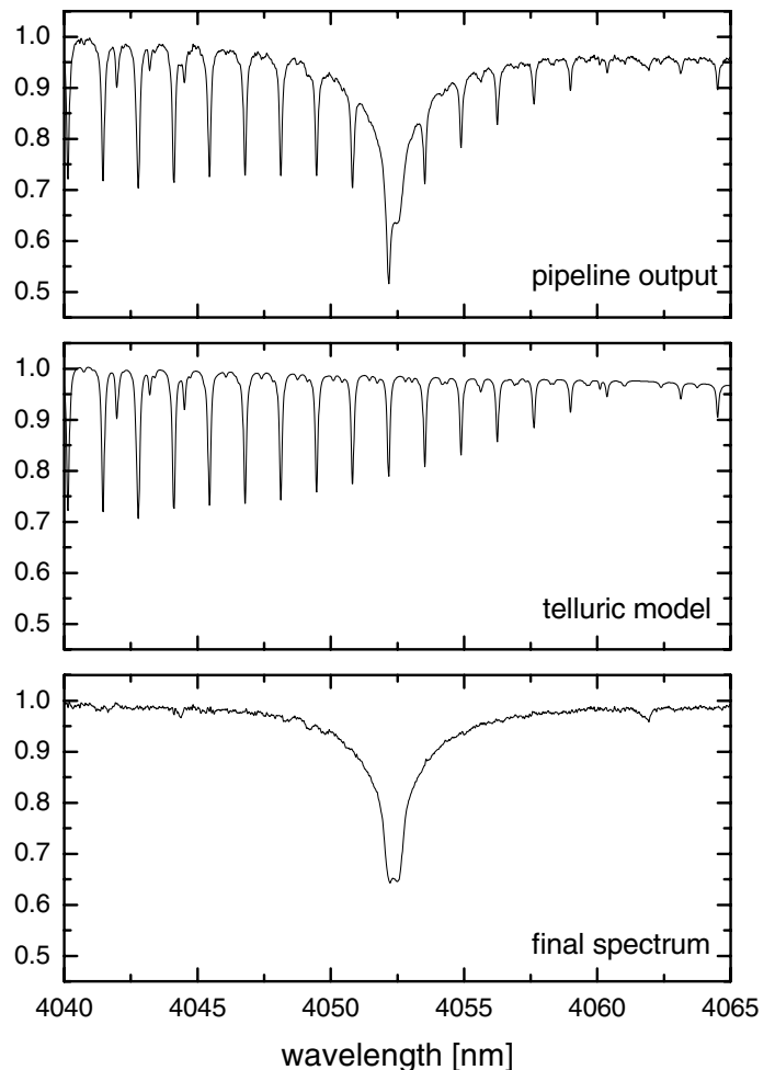
Fig. 2. Example of our method of correcting for the telluric absorption. The top panel shows the spectrum of HD 73634 (A6 II) around the Br- \alpha line at the level of the CRIFES pipeline data product after merging of two slightly overlapping spectral regions. The middle panel shows the telluric model calculated to fit the telluric lines in the observed spectrum. The bottom panel shows the resulting spectrum after division by the telluric spectrum and the application of some basic cosmetic corrections. Note that the emission core in the broad hydrogen line is real and not a residual of a telluric line.
