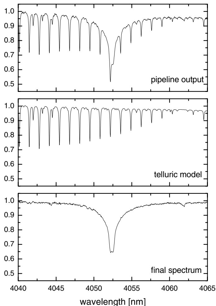
Fig. 2. Example of our method of correcting for the telluric absorption. The top panel shows the spectrum of HD 73634 (A6 II) around the Br- \alpha line at the level of the CRILES pipeline data product after merging of two slightly overlapping spectral regions. The middle panel shows the telluric model calculated to fit the telluric lines in the observed spectrum. The bottom panel shows the resulting spectrum after division by the telluric spectrum and the application of some basic cosmetic corrections. Note that the emission core in the broad hydrogen line is real and not a residual of a telluric line.
