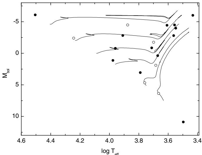
Fig. 1. Location of the CRIFES-POP stars in a HRD. Parameters taken from the literature or derived as described in the text. Filled symbols mark stars presented here, and open symbols the forthcoming objects. The solid lines indicate evolutionary tracks for solar-metallicity models of 10, 5, 3, 2, 1, and 0.6 M_{\odot} taken from Bertelli et al. (2008, 2009).
