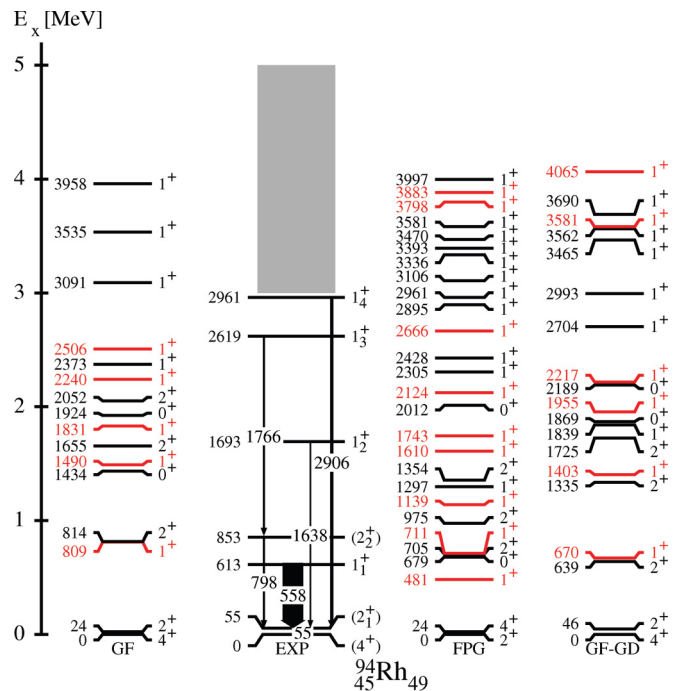
FIG. 2. (Color online) Deduced (EXP) and calculated (GF, FPG, GF-GD) level schemes for ^{94}\text{Rh} . Levels up to 4 MeV relevant for the \beta^+/EC decay are shown. The lowest two states in EXP correspond to ^{94m1}\text{Rh} and ^{94m3}\text{Rh} . See the text for details.
