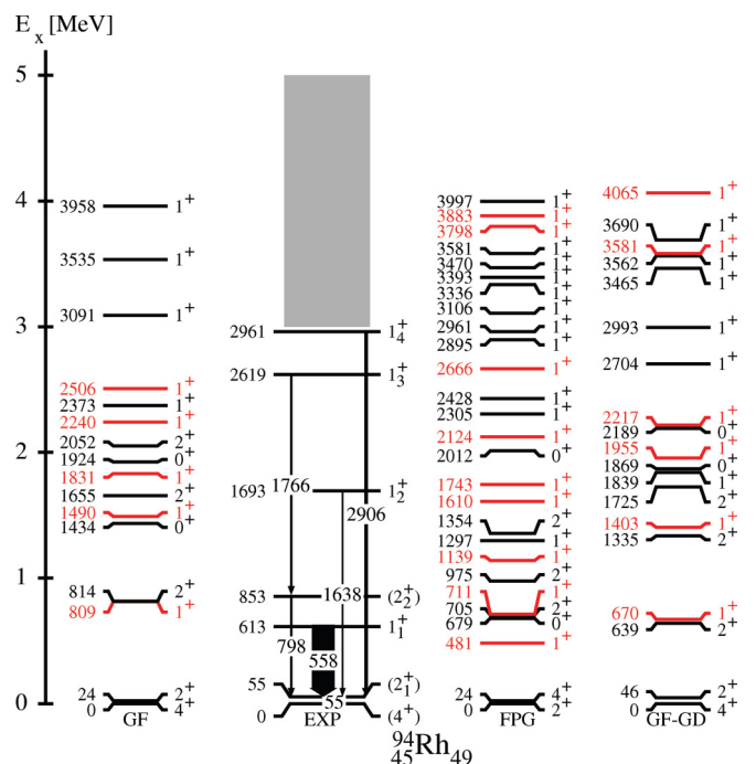
FIG. 2. (Color online) Deduced (EXP) and calculated (GF, FPG, GF-GD) level schemes for ^{94}\text{Rh} . Levels up to 4 MeV relevant for the \beta^+/\text{EC} decay are shown. The lowest two states in EXP correspond to ^{94m1}\text{Rh} and ^{94m3}\text{Rh} . See the text for details.
