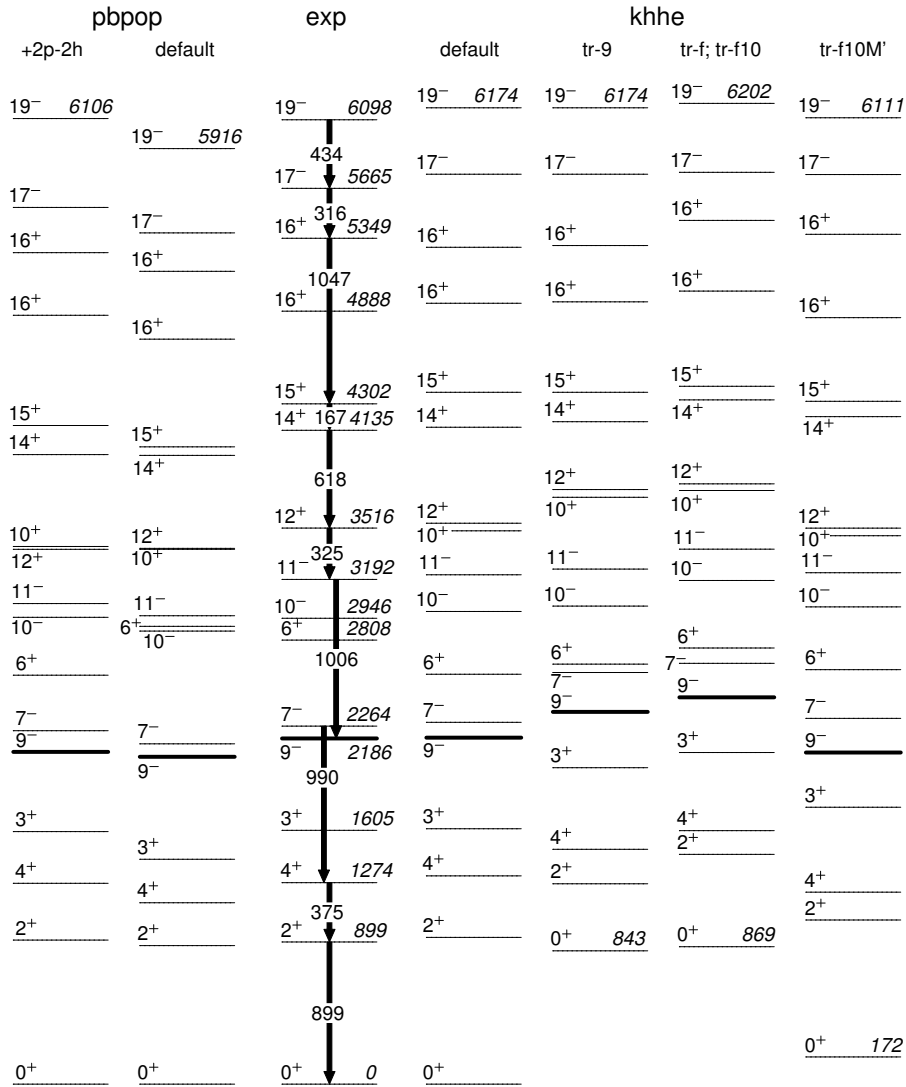
Figure 12. Comparison between experimental ('exp') [63] and predicted ('pbbop', 'khhe') decay schemes of ^{204}\text{Pb} starting from the 19^- isomer. Isomeric states are indicated by thick horizontal lines. All states are labelled with spin and parity, selected ones also with their excitation energy in keV. The main experimental \gamma -ray cascade is included for reference. Both 'pbbop' and the 'khhe default' calculations are normalized to the 0^+ ground state, the other 'khhe' schemes are presented relative to the 'default' ground state.
