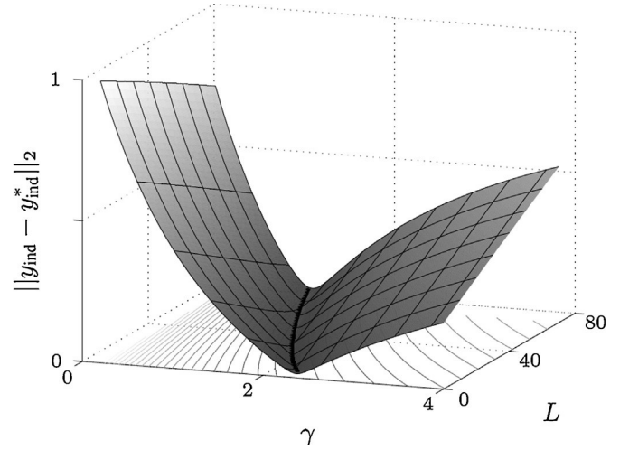
Fig. 7. Normalized L_2 -norm of induction phase output error as function of T and L .
