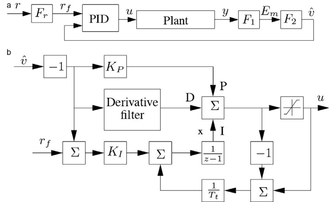
Fig. 6. Closed-loop system and PID controller.
