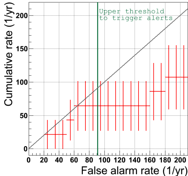
Fig. 14. Cumulative rate of triggers observed during the production period (excluding hardware injections) as a function of the upper threshold applied on the estimated false alarm rate.
