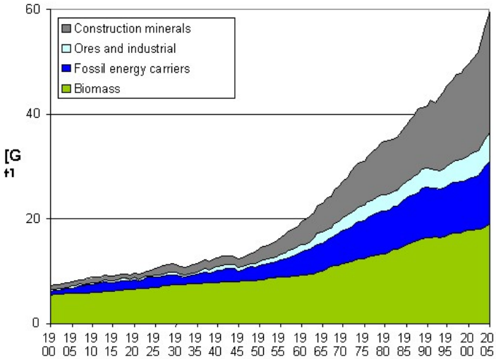
Figure 1.2. Global materials extraction 1900-2005, billion tons
