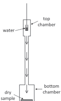
Fig. 3. Schematic graphic of the sorption ampoule. A dry sample is loaded in the bottom chamber and water is injected in the top chamber, where thermal power of sorption ( P_{\text{sorp}} ) and thermal power of evaporation ( P_{\text{vap}} ) are continuously measured by two twin microcalorimeters, respectively.
