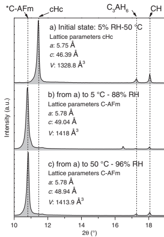
Fig. 9. XRD patterns of a sample initially containing cHc, hydrogarnet ( C_3AH_6 ) and portlandite (CH), and subsequently exposed to high RH at 5 and 50 °C. Shift of the main reflection towards lower 2\theta indicates higher water content. *C-AFm refers to a carbonated AFm phase of unknown composition.
