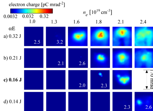
FIG. 1. Electron beam profiles for various plasma densities for different values of the amount of laser energy within the FWHM of the focal spot. (a), (b), and (d) kept the total laser energy constant but varied \alpha whereas (c) reduced the laser energy. Each panel is an average of five shots and is displayed on a logarithmic color scale.
