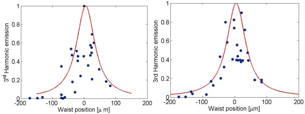
Figure 4: Total harmonic yield for 3 rd harmonic for low contrast( 10^{-7} ) (left) and high contrast ( 10^{-8} ) (right) of the incident laser pulse. Red lines indicate the Gaussian fit for the incident laser pulse intensity.
