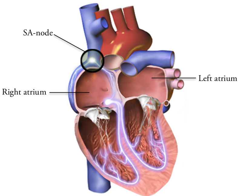
Figure 1.1. Electrical impulses normally originates from the sinoatrial (SA) node in the right atrium. In atrial fibrillation, this electrical activity is disturbed. Copyright © Blausen Medical Communications, Inc.
