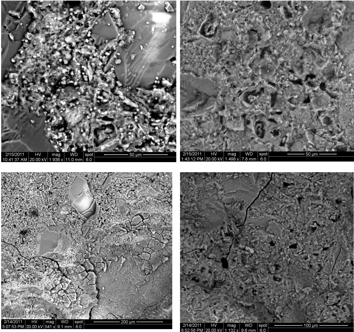
Figure A3.3: Specimens exposed to water suction from the un-cracked side. Cover 55 mm. Left column: 5 mm from crack mouth. Right column: 50 mm from crack mouth. Upper row: Crack width 0.2 mm; Specimen H55-2-3-2. Lower row: Crack width 0.4 mm; Specimen H55-4-3-2.
