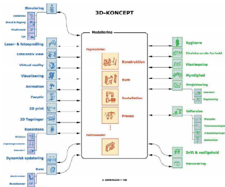
Figur 9. Rambølls 3D-koncept/model.
