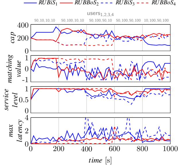
Figure 7: Resource manager and four applications.
