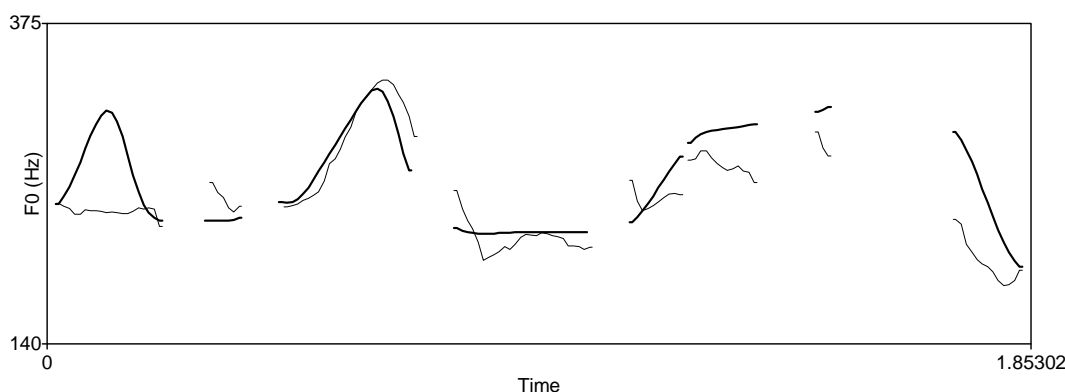
Figure 7. Modified f_0 course of the sentence ↑Он ↑не понимает ↑↑элементарных ↓↓вещей. on n'e ponimájet elementárnix v'eshčej 'He does not understand simple things.' Female speaker.
