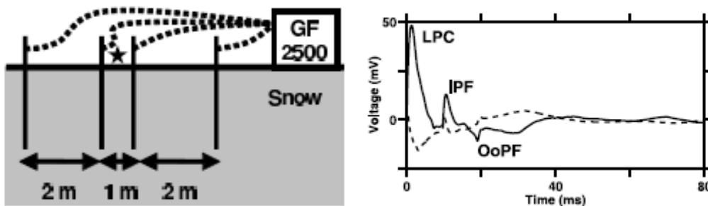
Figur 8.15. Dipolarrangemang kring skottpunkten (*) t.v. Mottagna signaler t.h. Helt dragen respektive streckad linje från ömse sidor av skottpunkten. Dipole arrangement around the shotpoint (*) (left). Received signals (right). Solid and dashed lines represent signals from either side of the shotpoint.
