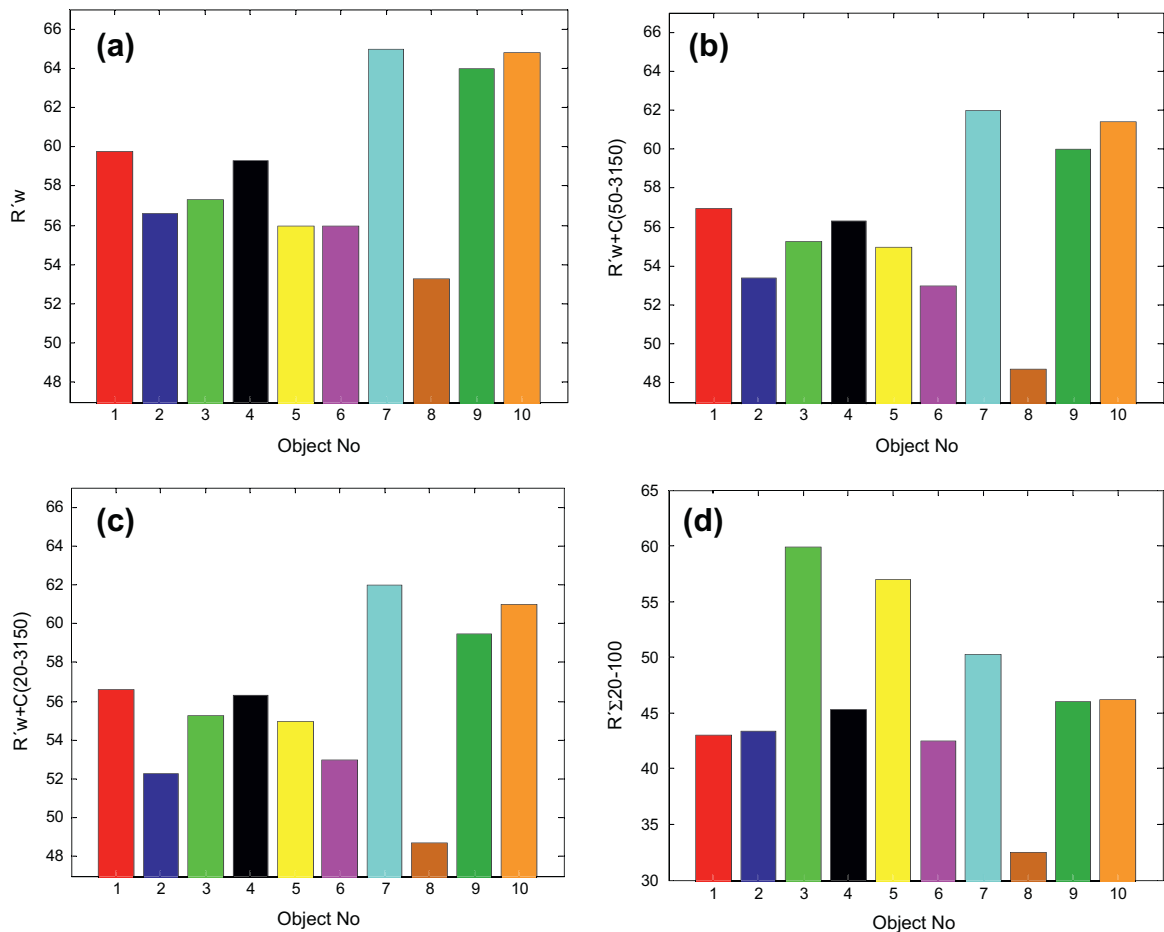
Fig. 1. Airborne sound insulation; (a) R'_w , (b) R'_w + C_{50-3150} , (c) R'_w + C_{20-3150} and (d) R'_w + C_{20-100} .
