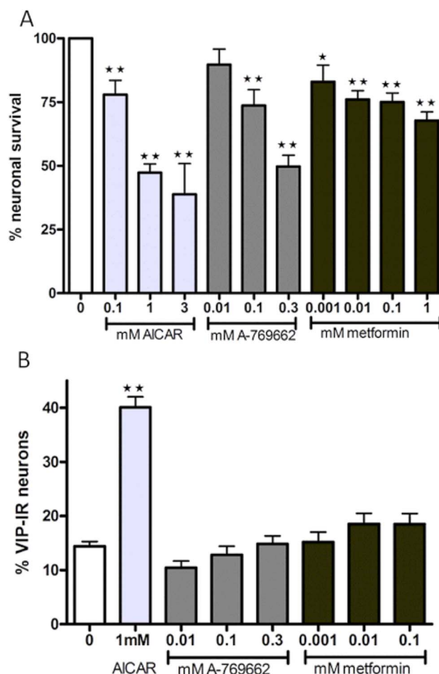
Figure 3. Effects of AMPK activation on survival and relative numbers of VIP-immunoreactive (IR) myenteric neurons. A. Neuronal survival, expressed as % of controls, after 4 days of exposure to AICAR ( 10^{-4} – 3 \times 10^{-3} M), A-769662 ( 10^{-5} – 3 \times 10^{-4} M) or metformin ( 10^{-6} – 10^{-3} M). Nerve cell bodies were identified using immunostaining against HuC/HuD. AICAR, A-769662 and metformin induced a concentration dependent loss of neurons. B. shows the relative numbers of VIP-IR neurons, expressed in percentage of HuC/HuD-IR neurons, after exposure to AICAR ( 10^{-3} M), A-769662 ( 10^{-5} – 3 \times 10^{-4} M) or metformin ( 10^{-6} – 10^{-3} M). AICAR increases the relative numbers of VIP-IR neurons while A-769662 and metformin does not, compared to control. Data expressed as mean \pm SEM, ** p < 0.01 , n = 4 –24.
