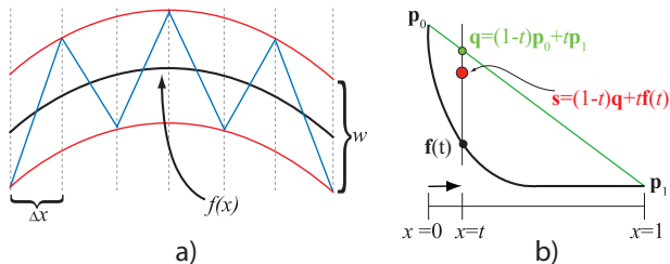
Figure 5: We must take special care of the interval remainder term when performing backface culling. Figure a) shows a worst case derivative of a Taylor model with a polynomial f(x) an interval remainder term with width w . The worst case derivative that can be introduced by the remainder term is given by the blue sawtooth pattern, which has a period of 2\Delta x where \Delta x is the length of the shortest edge created during tessellation. Figure b) shows how we alter the original fractional tessellation algorithm to avoid problems that would arise in Figure a) if \Delta x is very small.
