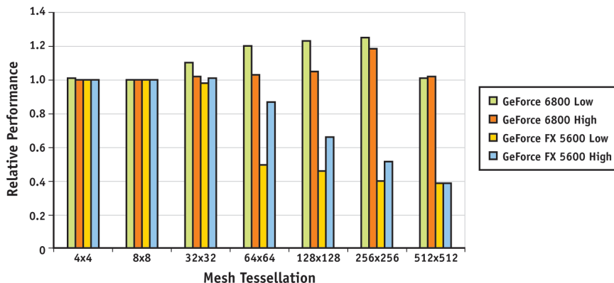
Figure 7: Benchmarked Results: Benchmarks on a GeForce 6800 Series GPU and a GeForce FX 5600. Tests were performed at low ( 128 \times 128 pixels) and high ( 1024 \times 1024 pixels) resolution. The graph shows the relative performance of the first algorithm compared to the second.
