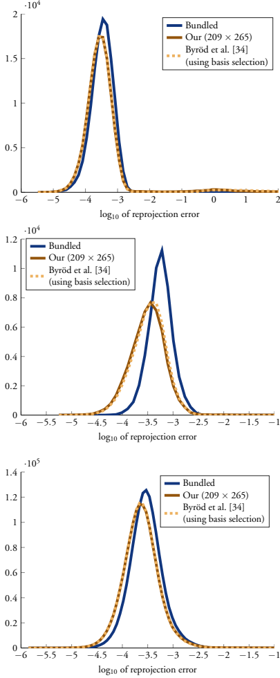
Figure 2.4: Triangulated points for three real problems using our triangulation method. Top to bottom: the Notre Dame dataset [195] with around 120,000 3D-points, the Orebro Castle dataset [174] (around 50,000 3D-points), and the Arts Quad dataset [45] (around 1,400,000 3D-points). Histograms show reprojection errors for our method compared to the solutions provided in the original datasets (which are bundled over all available cameras, hence the slightly larger median error) and the solver from [34].
