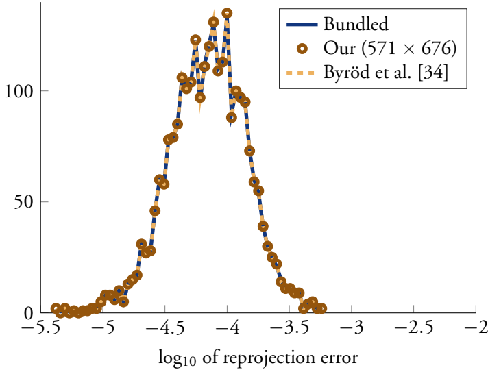
Figure 2.2: Error histograms for the dinosaur experiment for the different methods, on a log-scale.
