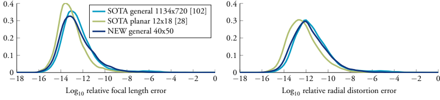
Figure 5.3: Histograms of \log_{10} relative errors of the estimated focal lengths (left) and radial distortions (right) for planar scenes.
