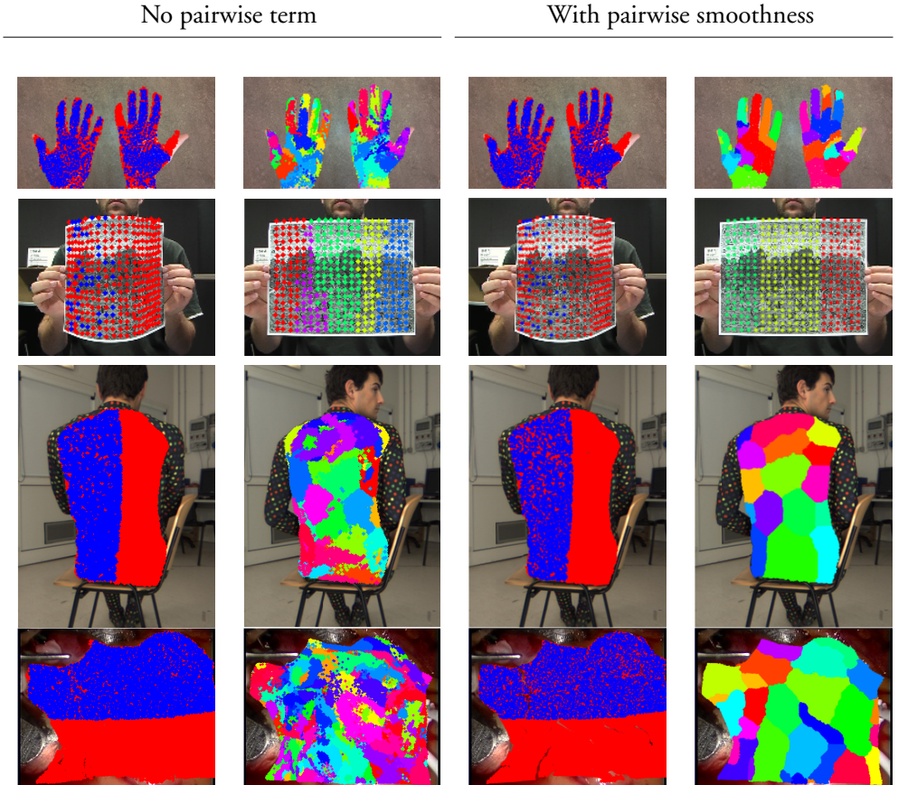
Figure 8.11: Estimated point positions and obtained clusters using the energy (8.17) with and without the smoothness term S_{pq} .
