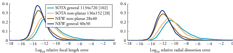
Figure 5.2: Histograms of \log_{10} relative errors of the estimated focal lengths (left) and radial distortions (right) for non-planar scenes.
