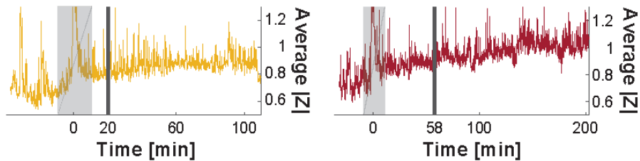
Figure 9. Averaged absolute deviations from mean baseline firing rates for all experiments with D1R antagonist (left, yellow) and D2R antagonist (right, maroon). Significant rate changes are observed shortly after administration of drugs preceding the first evidence of catalepsy.
