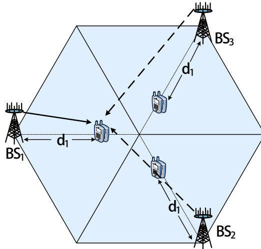
Figure 1: An example of CoMP system, where the solid line denotes local channel while the dash lines denote cross channels for a MS. The cell radius is 250 m. The MSs in the same cell are co-located in the same place, and the user-groups in different cells are at the same distance from their local BSs.
