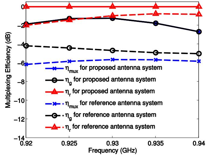
Fig. 14. Multiplexing efficiencies of the proposed and reference dual-antenna systems. \eta_{\text{mux}} and \eta_g for the proposed system almost overlap with each other.
